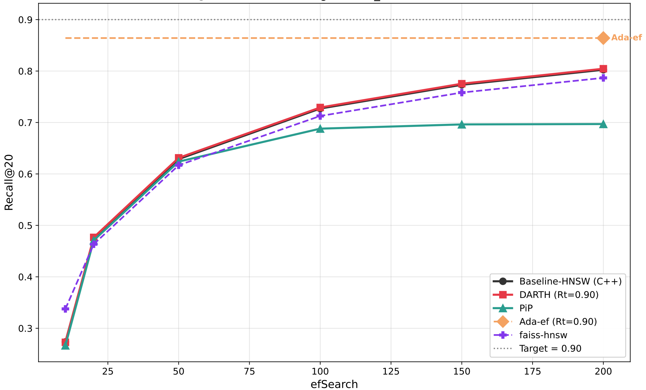
Recall@20 vs efSearch — glove100_full (M=16, efC=200)
