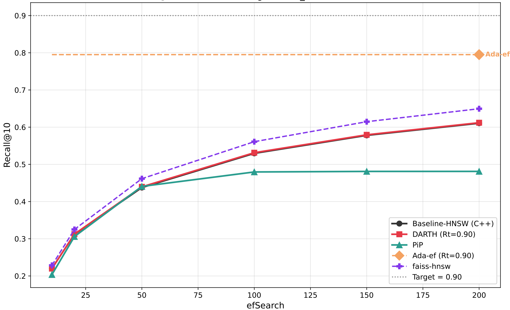
Recall@10 vs efSearch — glove100_full (M=8, efC=128)
