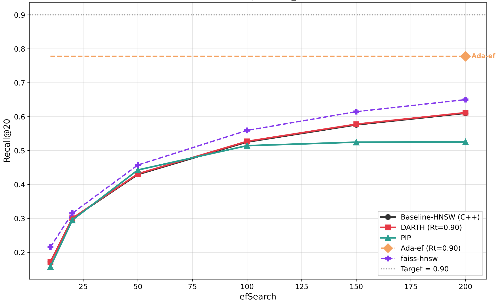
Recall@20 vs efSearch — glove100_full (M=8, efC=128)
