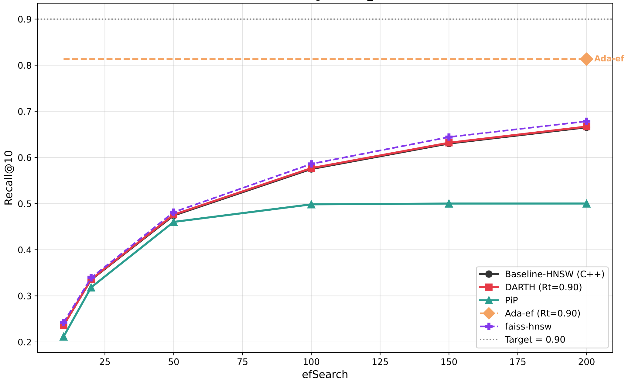
Recall@10 vs efSearch — glove100_full (M=8, efC=200)
