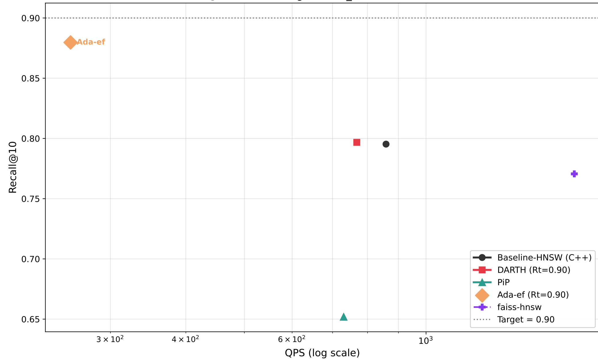
Recall@10 vs QPS — glove100_full (M=16, efC=128)
