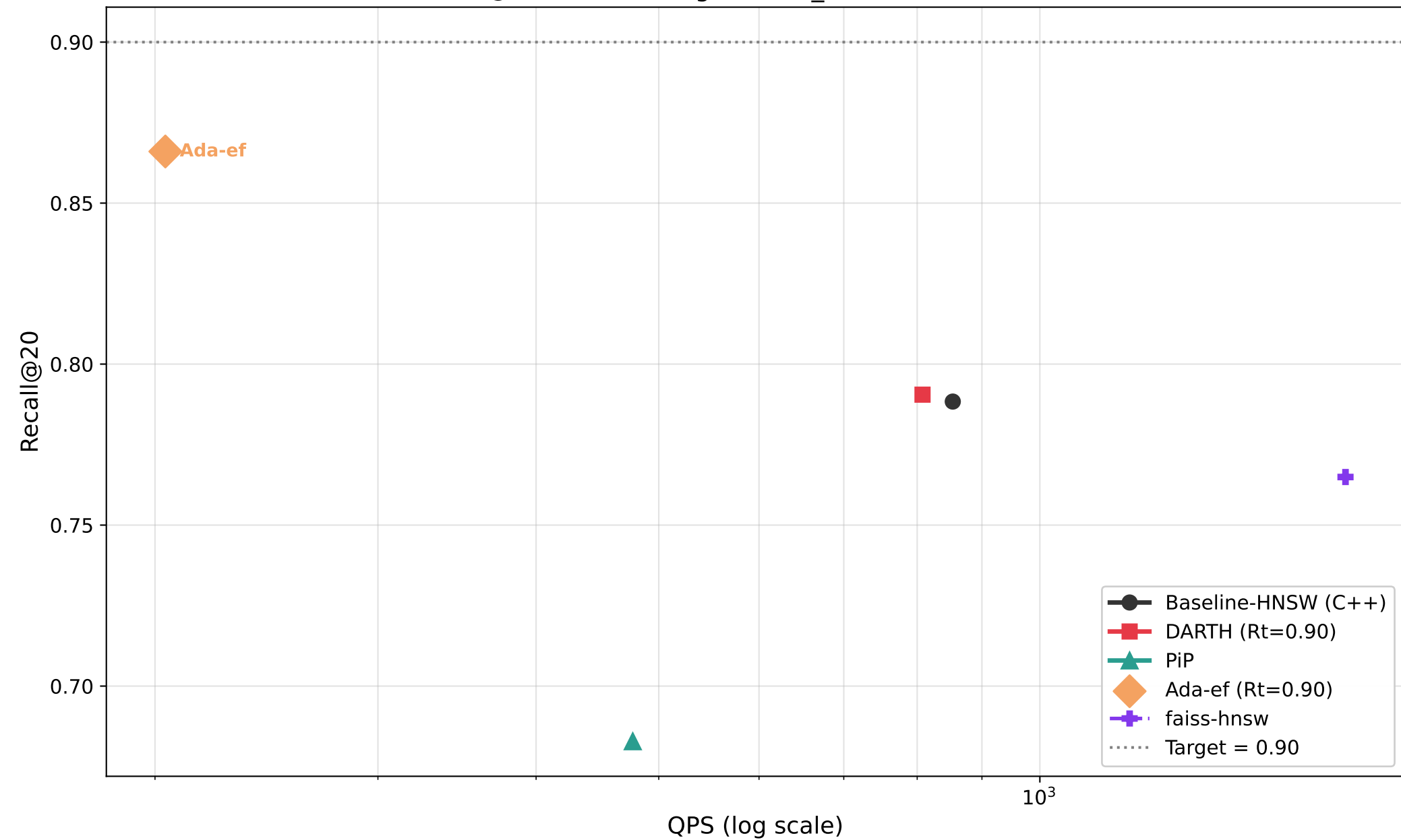
Recall@20 vs QPS — glove100_full (M=16, efC=128)
