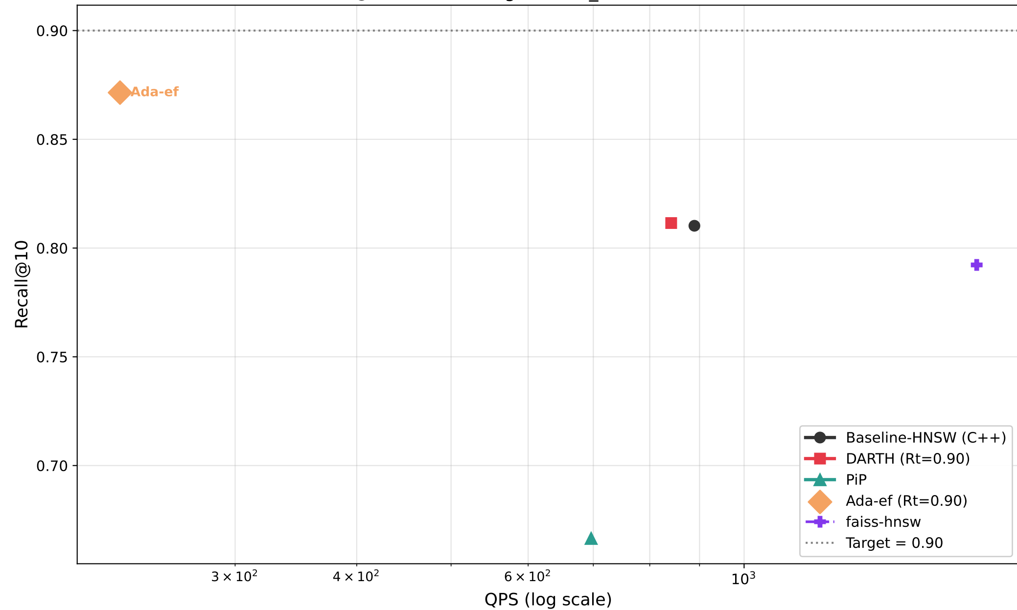
Recall@10 vs QPS — glove100_full (M=16, efC=200)
