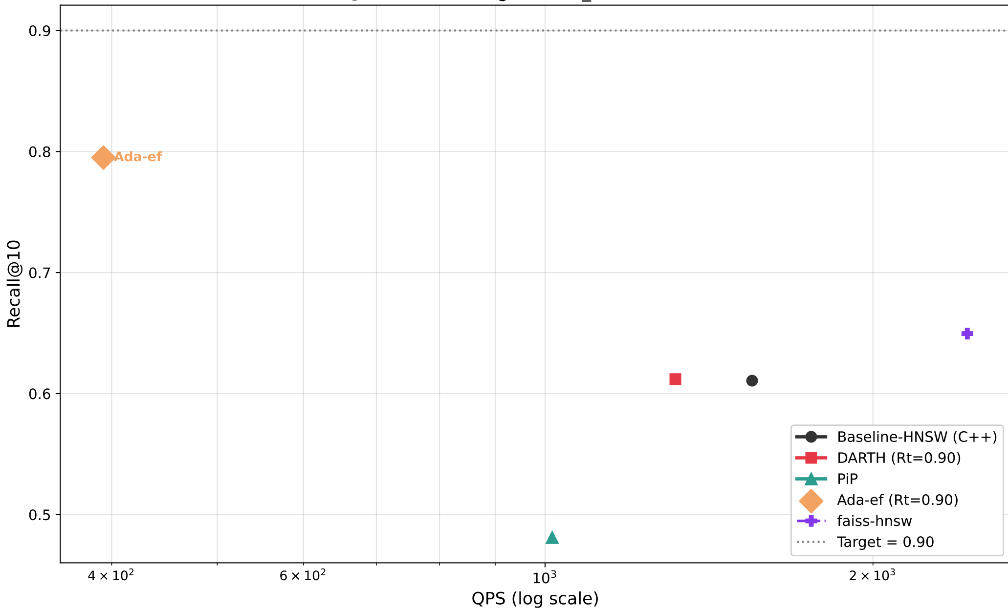
Recall@10 vs QPS — glove100_full (M=8, efC=128)
