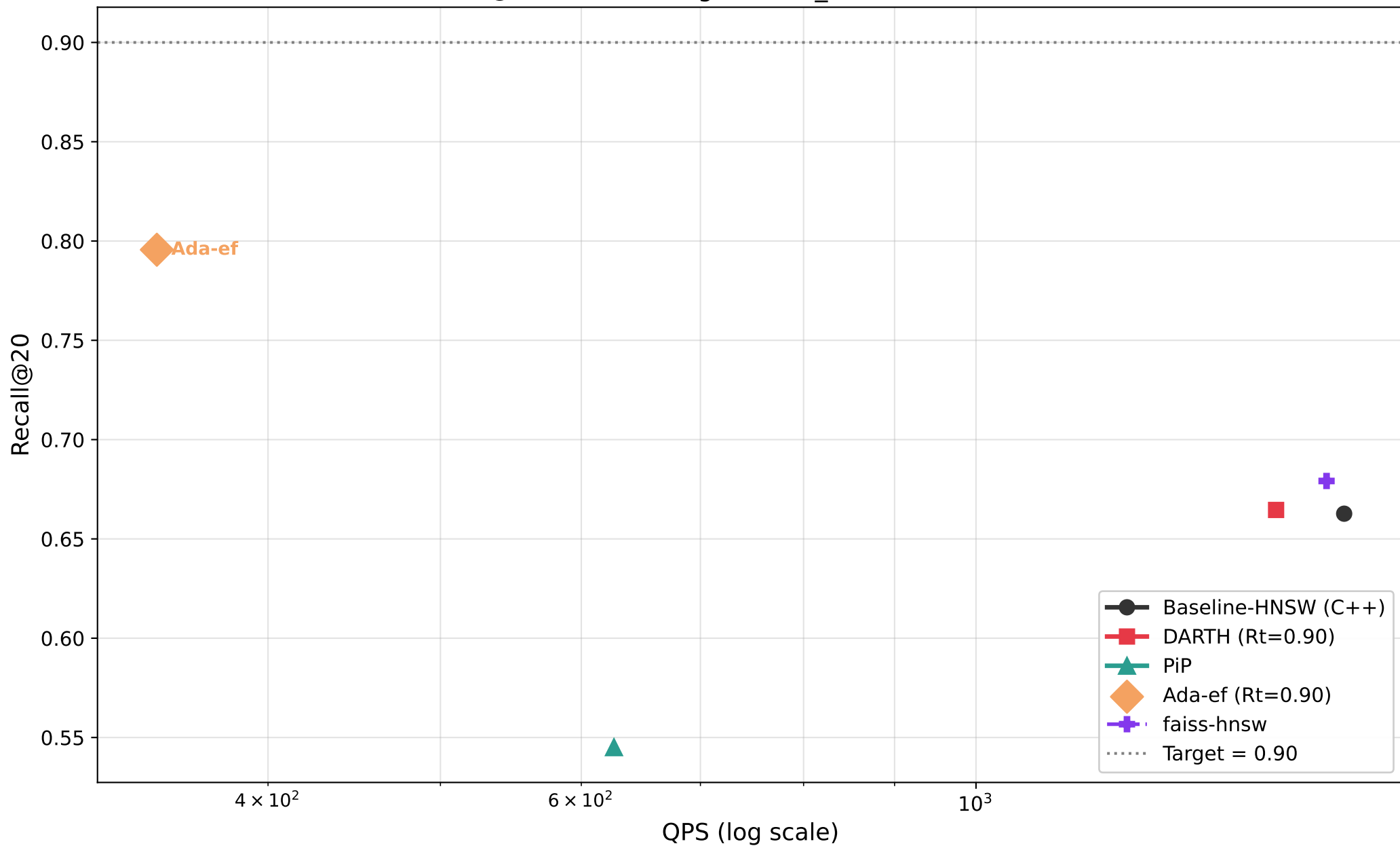
Recall@20 vs QPS — glove100_full (M=8, efC=200)
