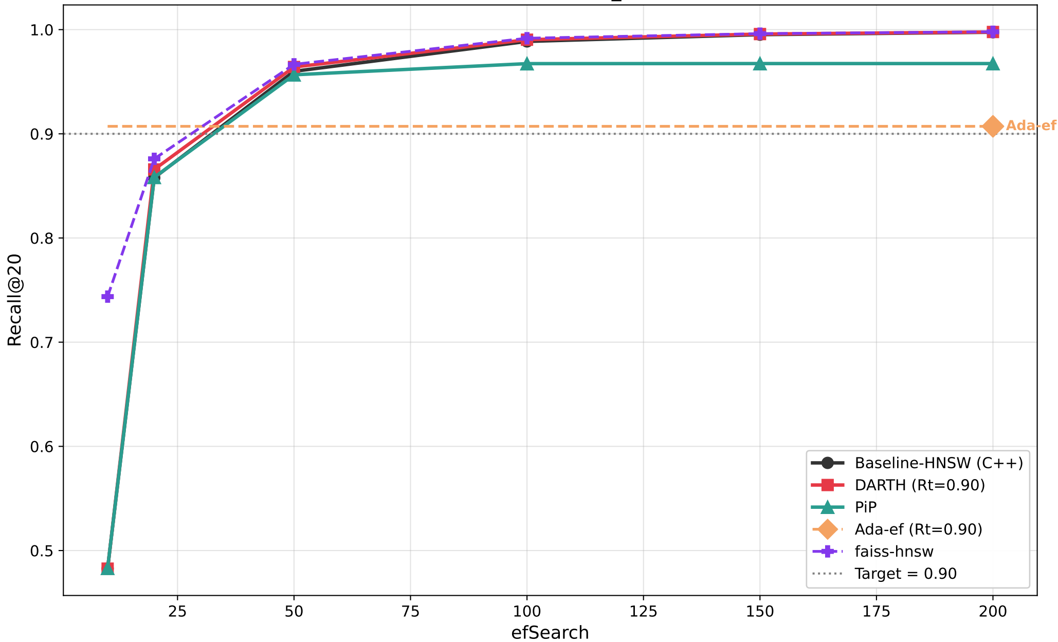
Recall@20 vs efSearch — msmarco_text (M=16, efC=200)
