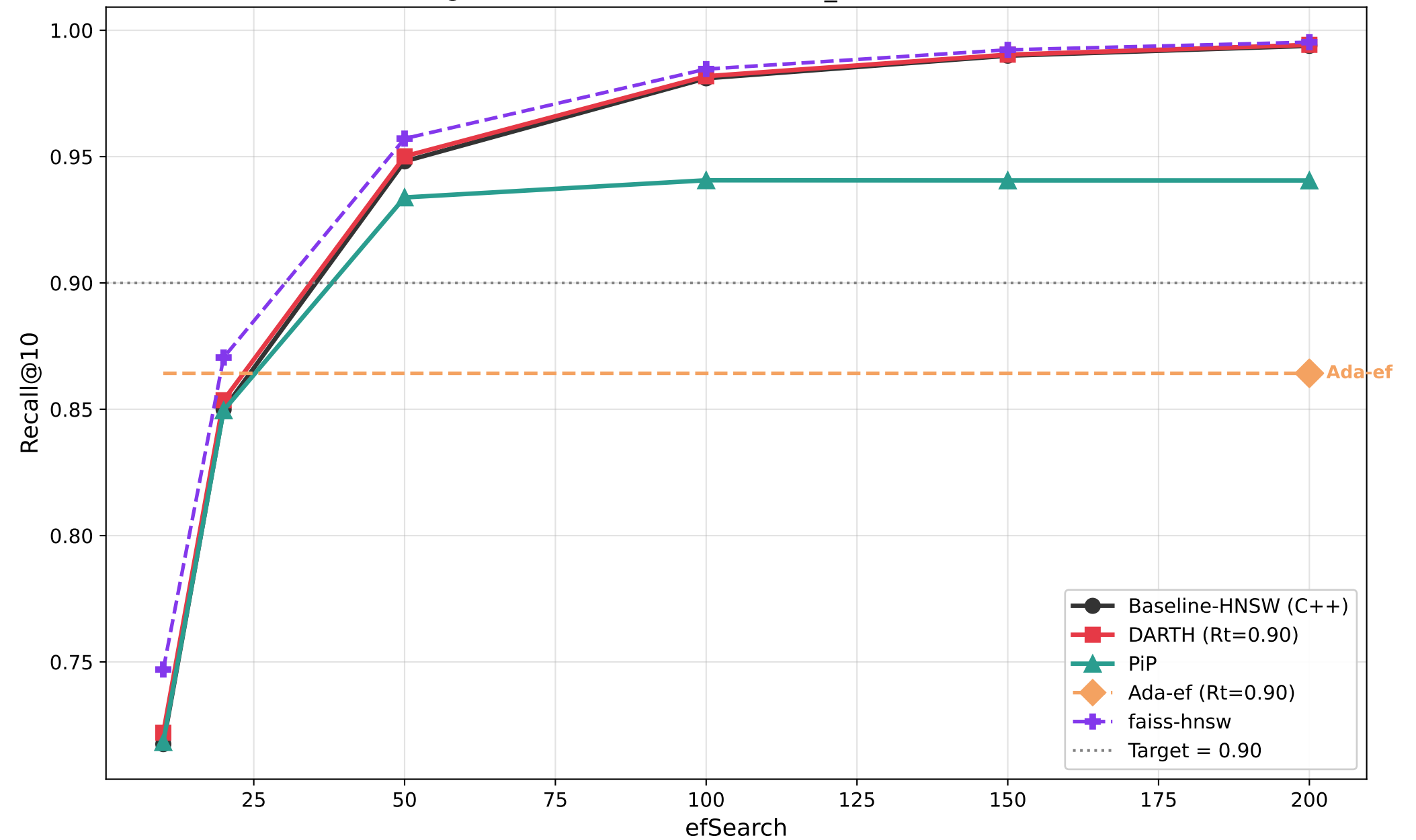
Recall@10 vs efSearch — msmarco_text (M=8, efC=200)
