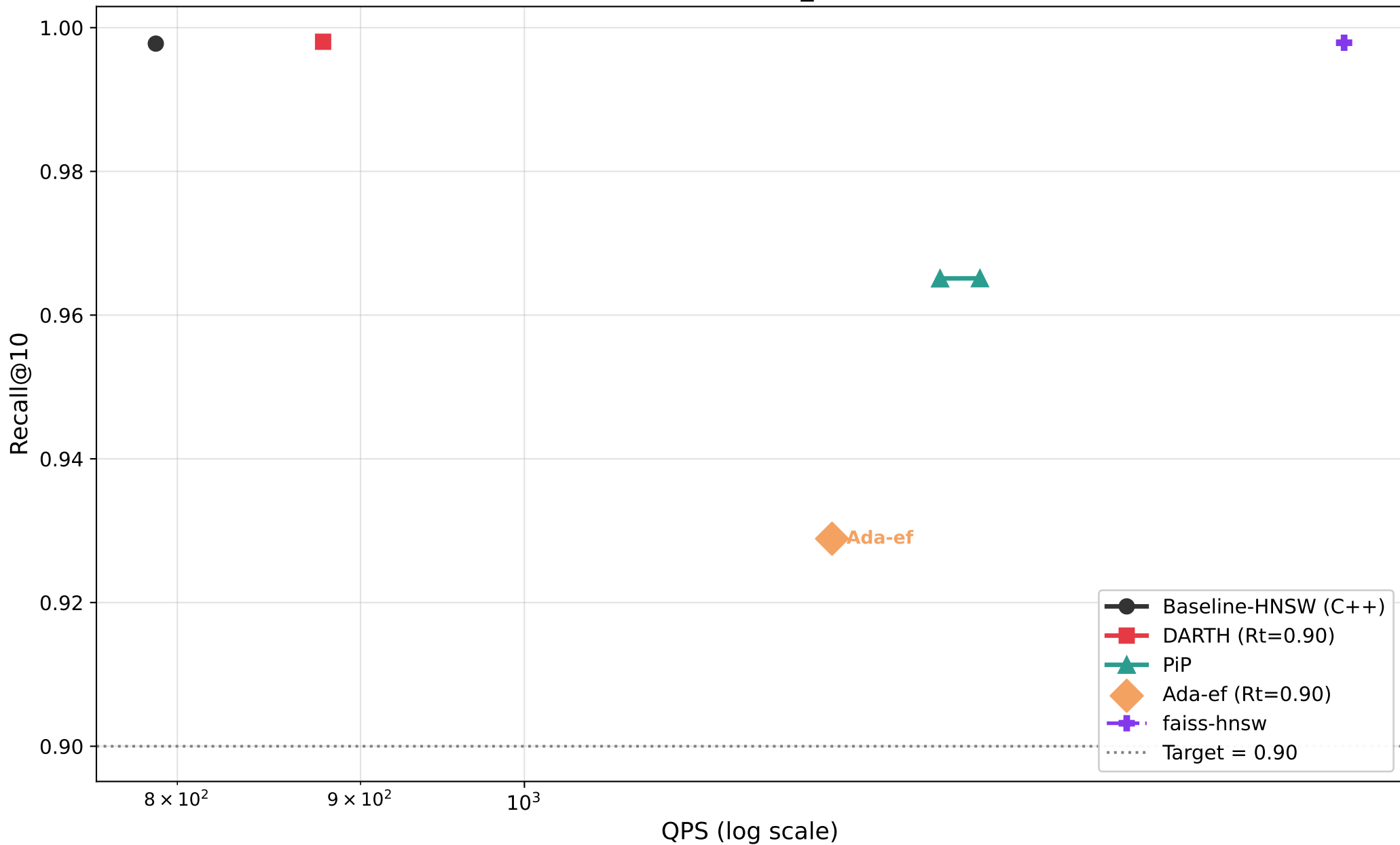
Recall@10 vs QPS — msmarco_text (M=16, efC=128)
