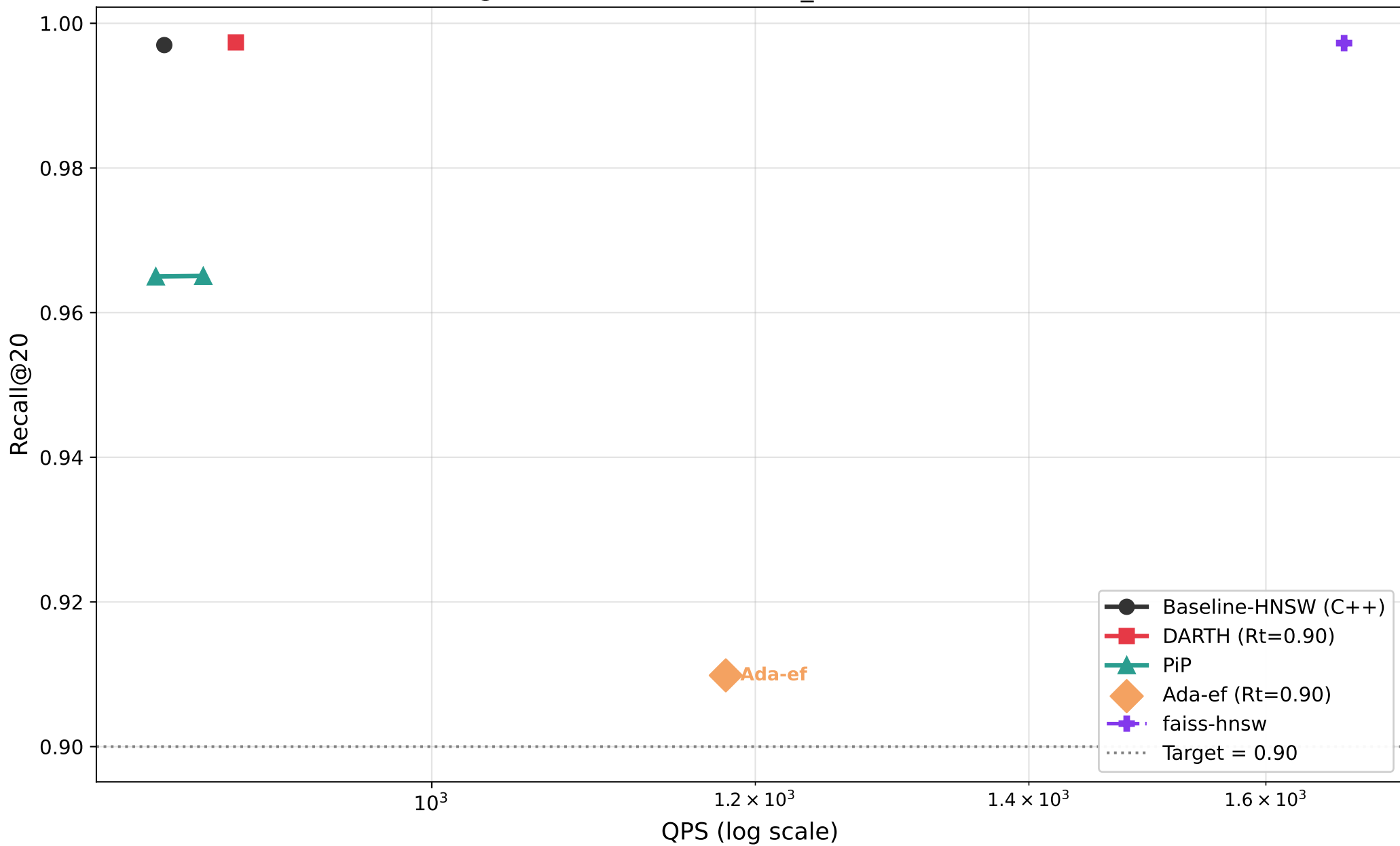
Recall@20 vs QPS — msmarco_text (M=16, efC=128)
