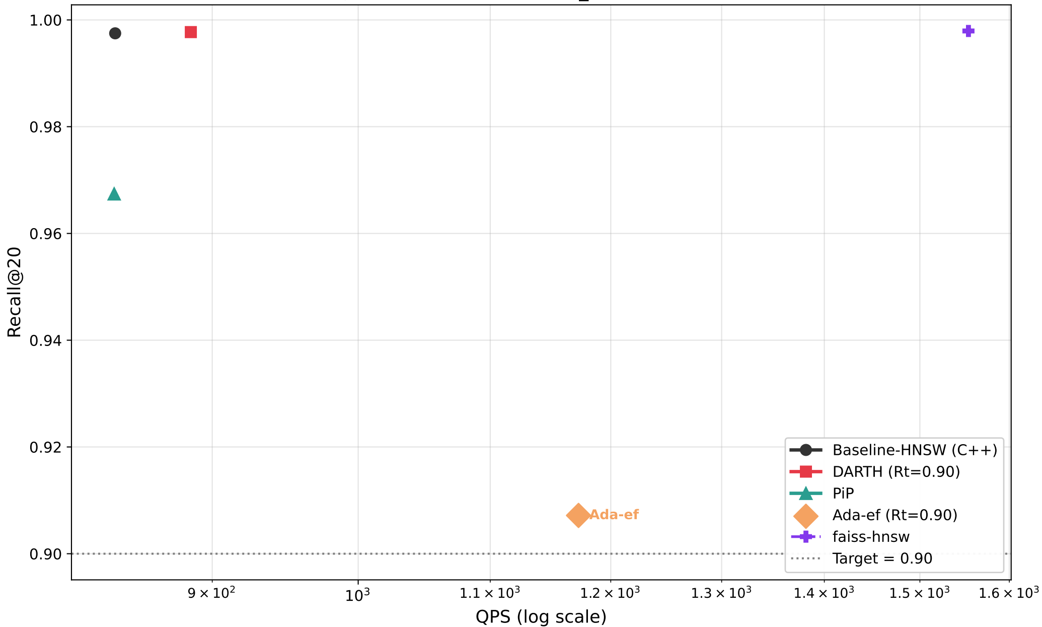
Recall@20 vs QPS — msmarco_text (M=16, efC=200)
