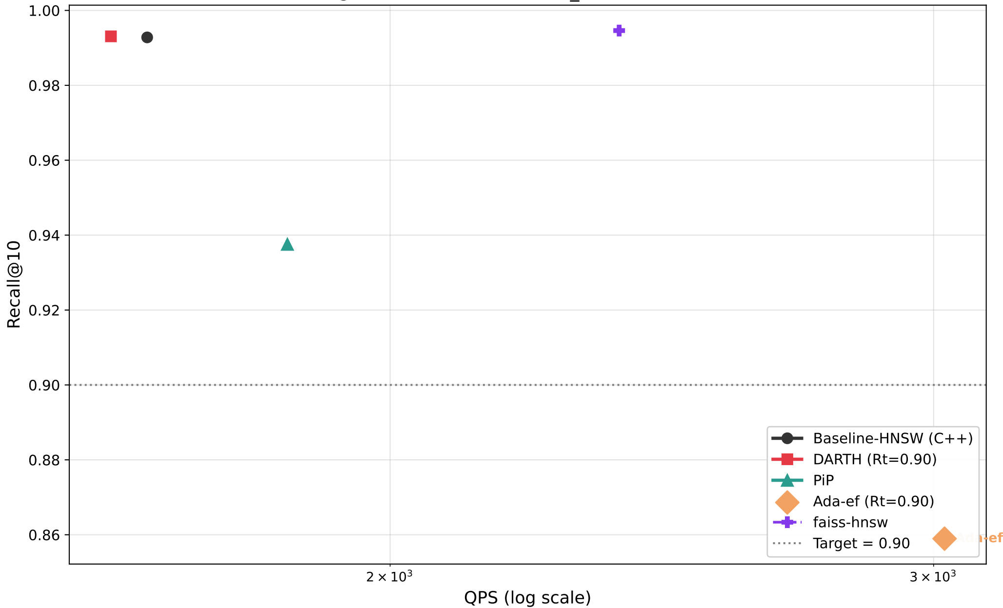
Recall@10 vs QPS — msmarco_text (M=8, efC=128)
