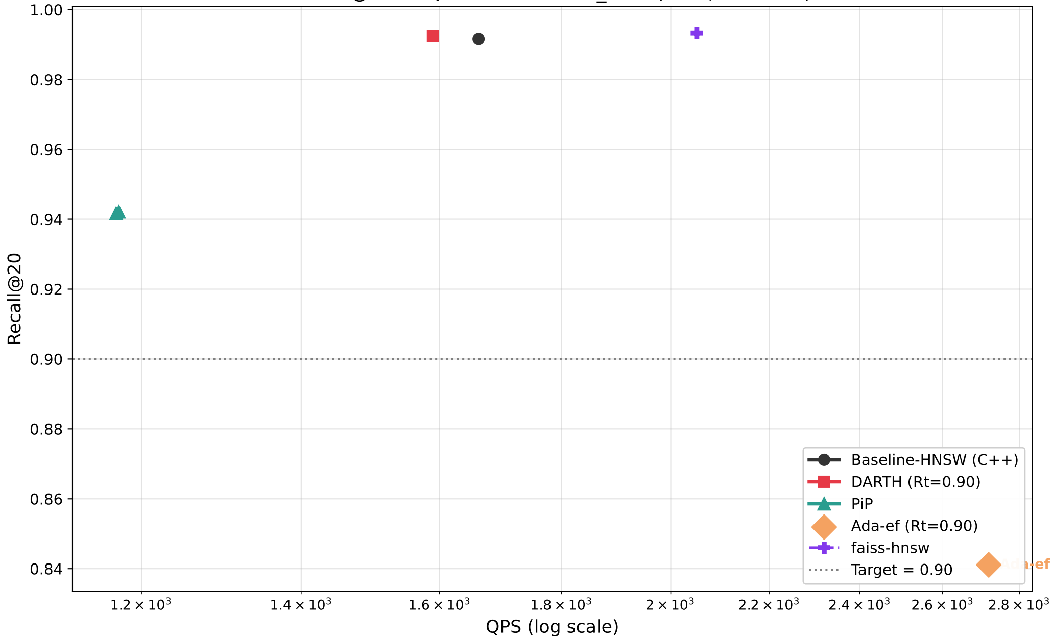
Recall@20 vs QPS — msmarco_text (M=8, efC=200)
