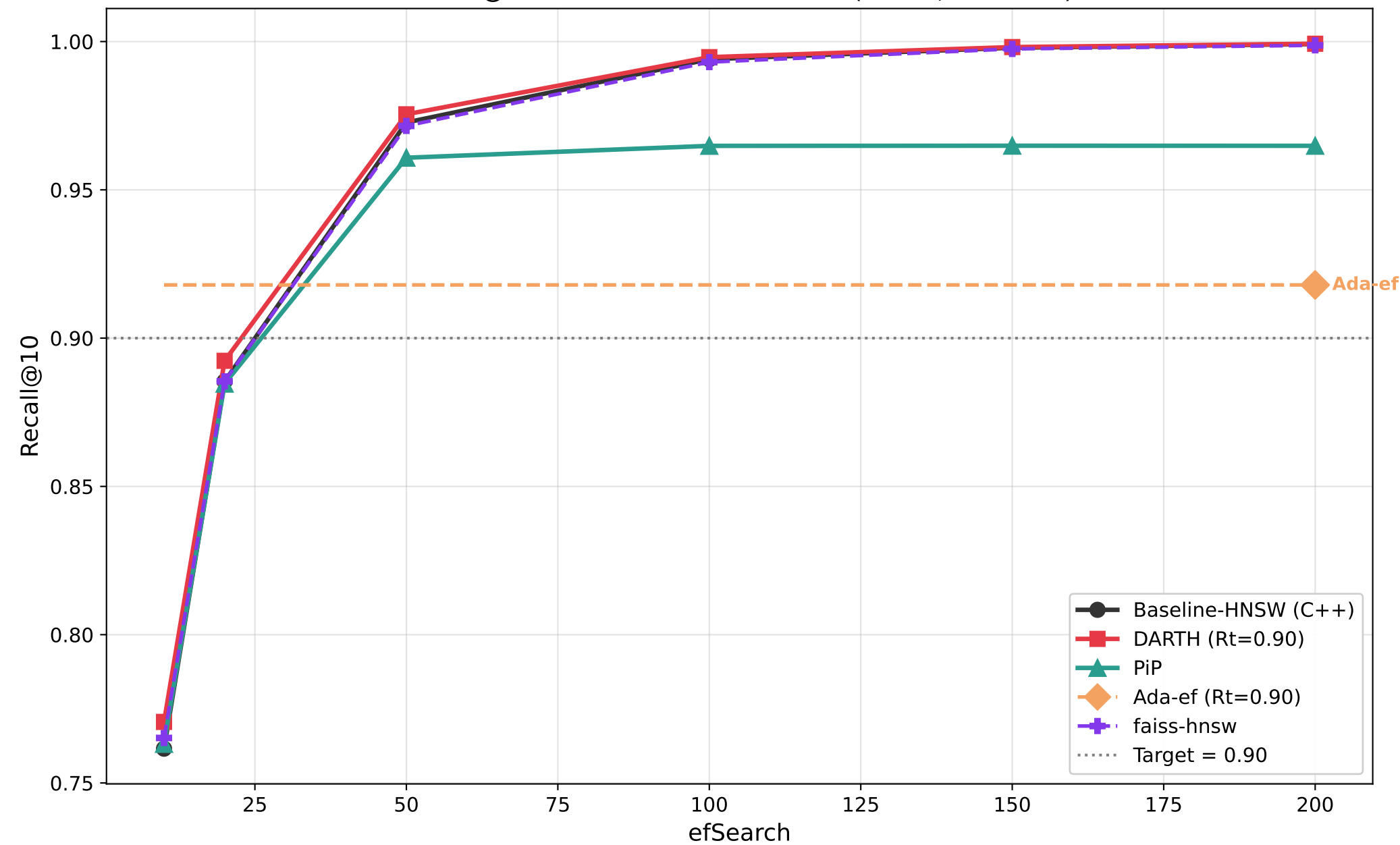
Recall@10 vs efSearch — sift128 (M=16, efC=128)
