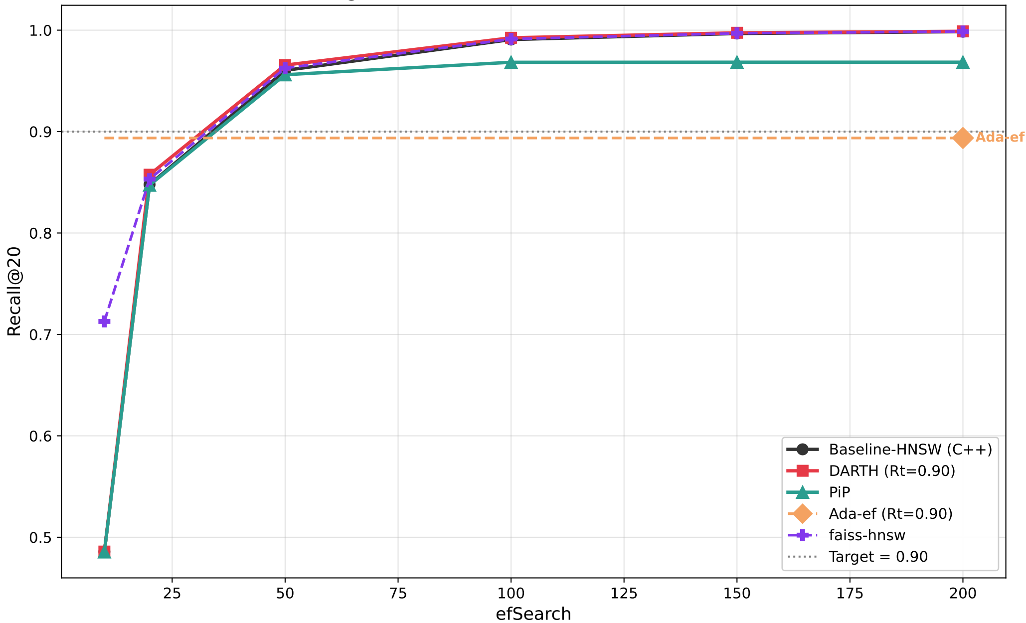
Recall@20 vs efSearch — sift128 (M=16, efC=200)
