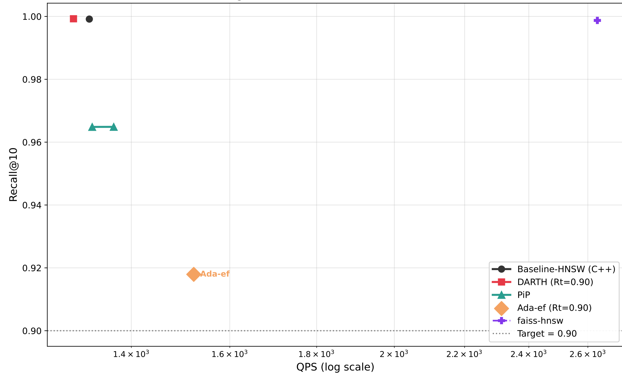
Recall@10 vs QPS — sift128 (M=16, efC=128)
