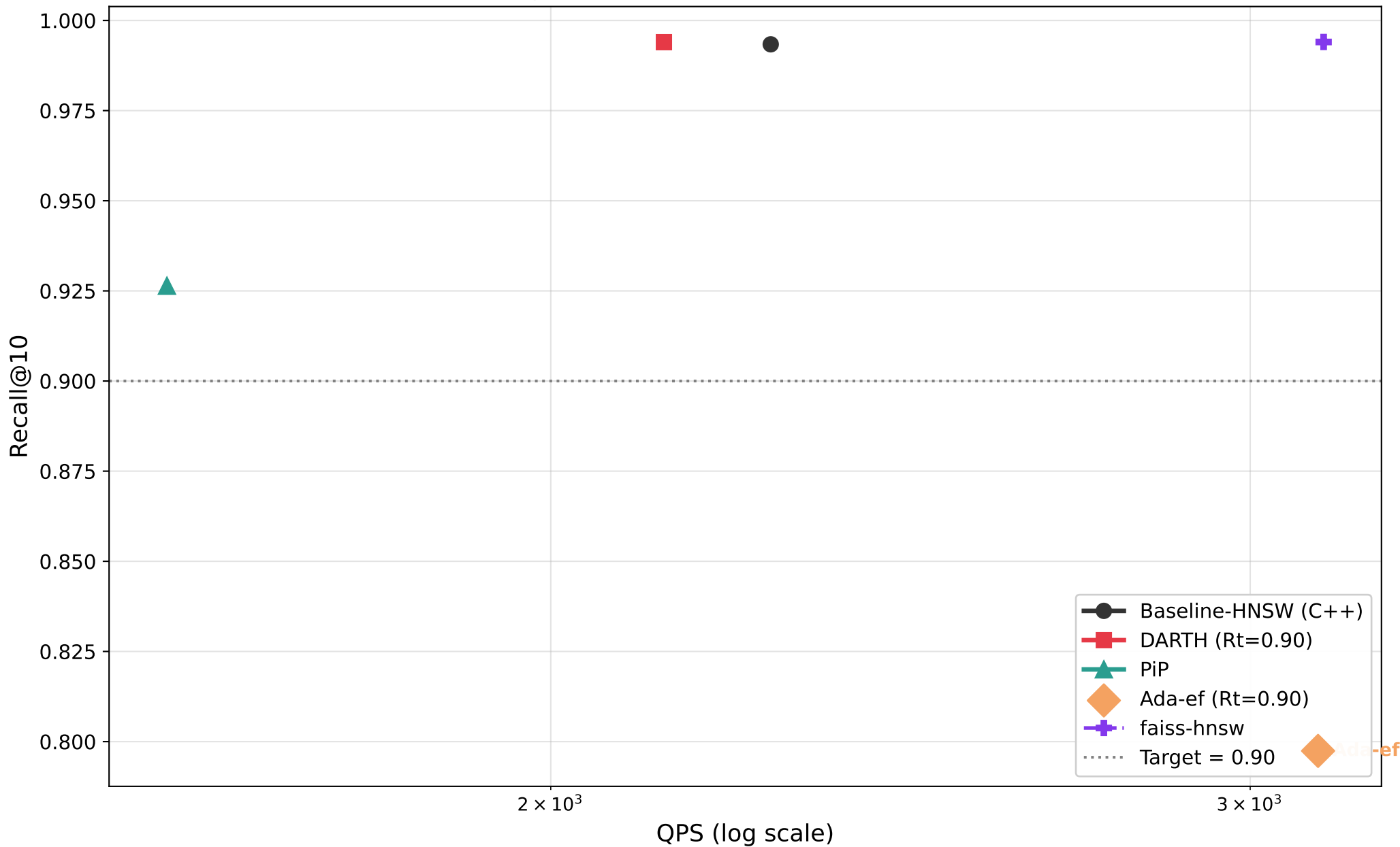
Recall@10 vs QPS — sift128 (M=8, efC=128)
