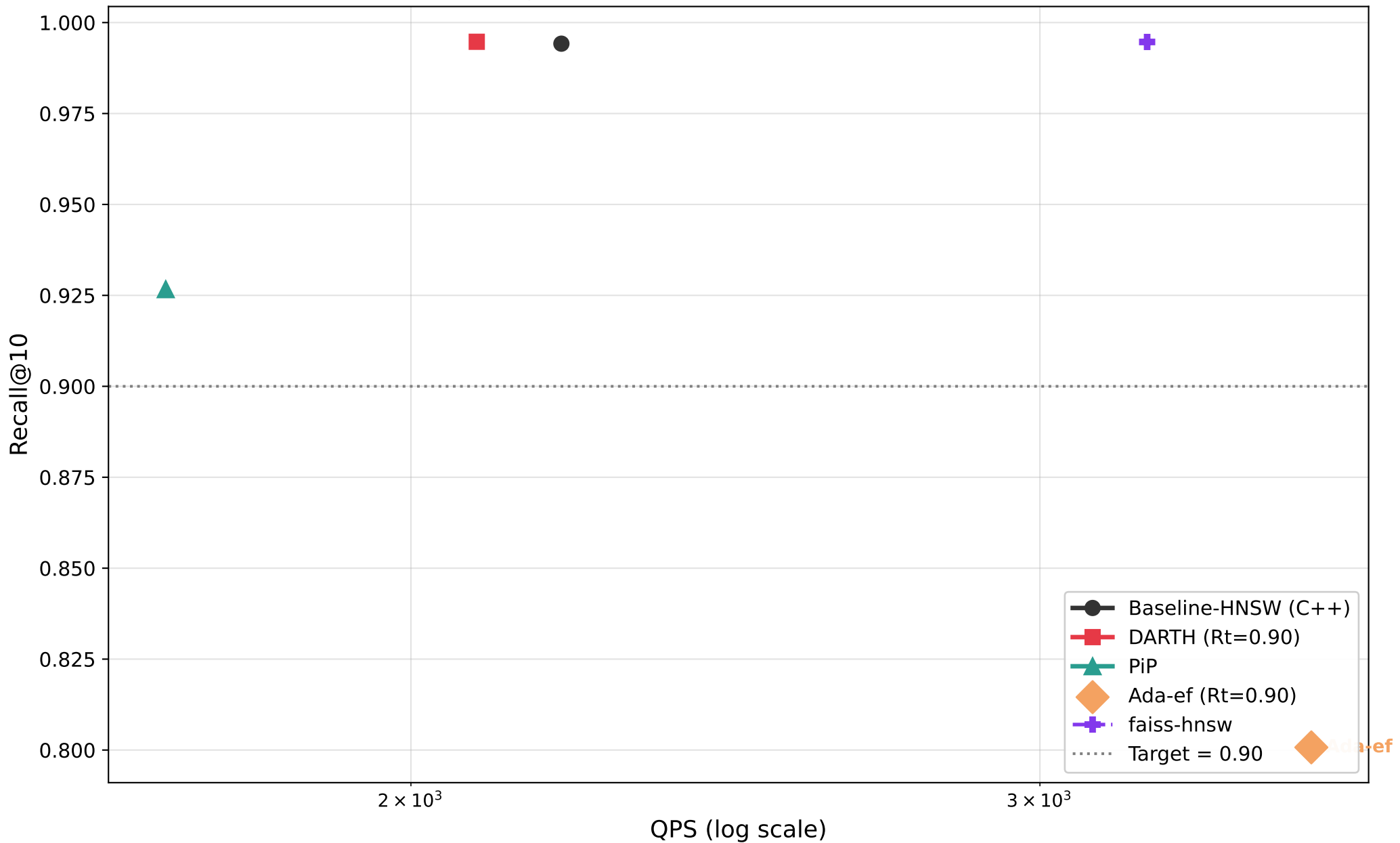
Recall@10 vs QPS — sift128 (M=8, efC=200)
