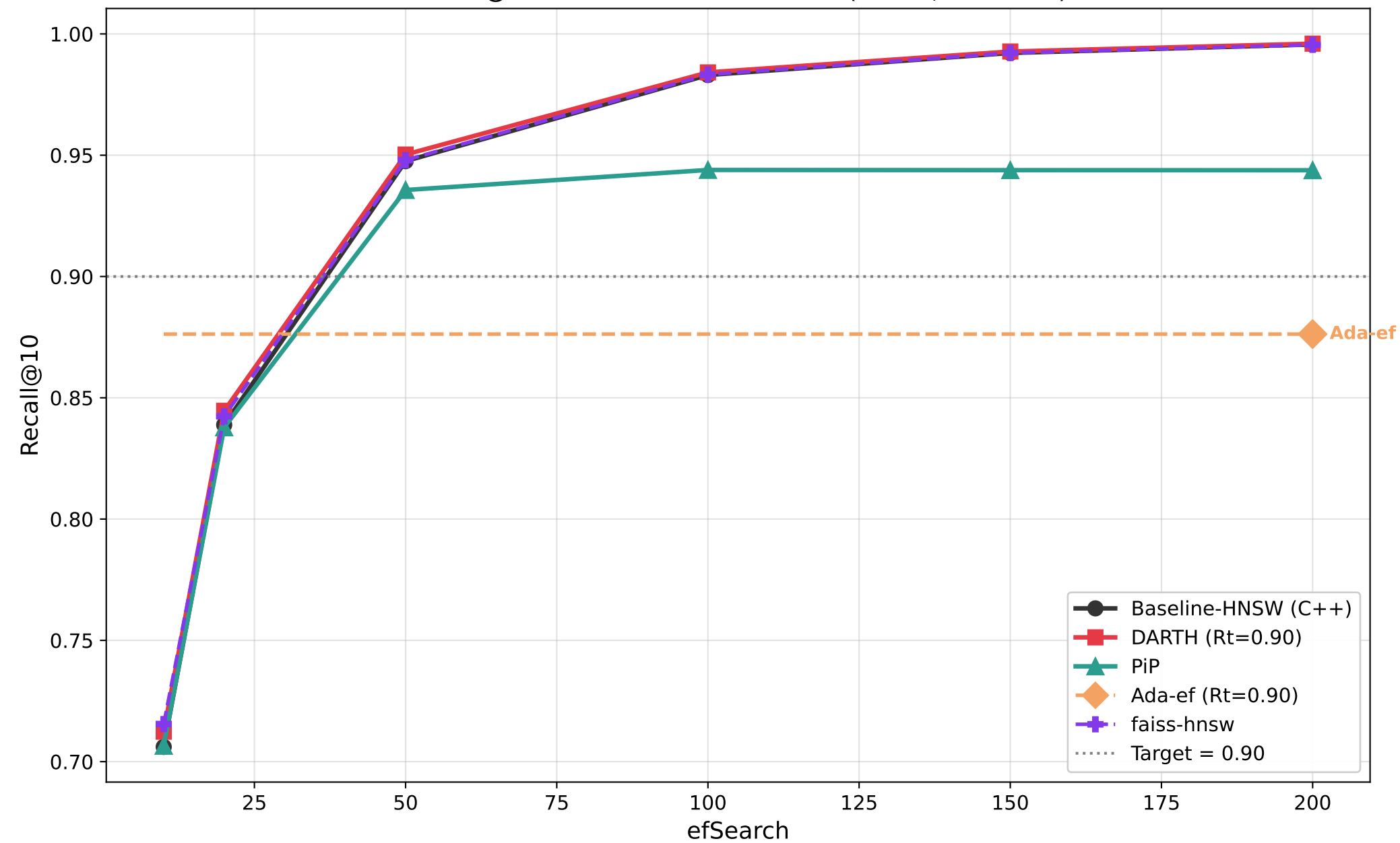
Recall@10 vs efSearch — sift1m (M=16, efC=128)
