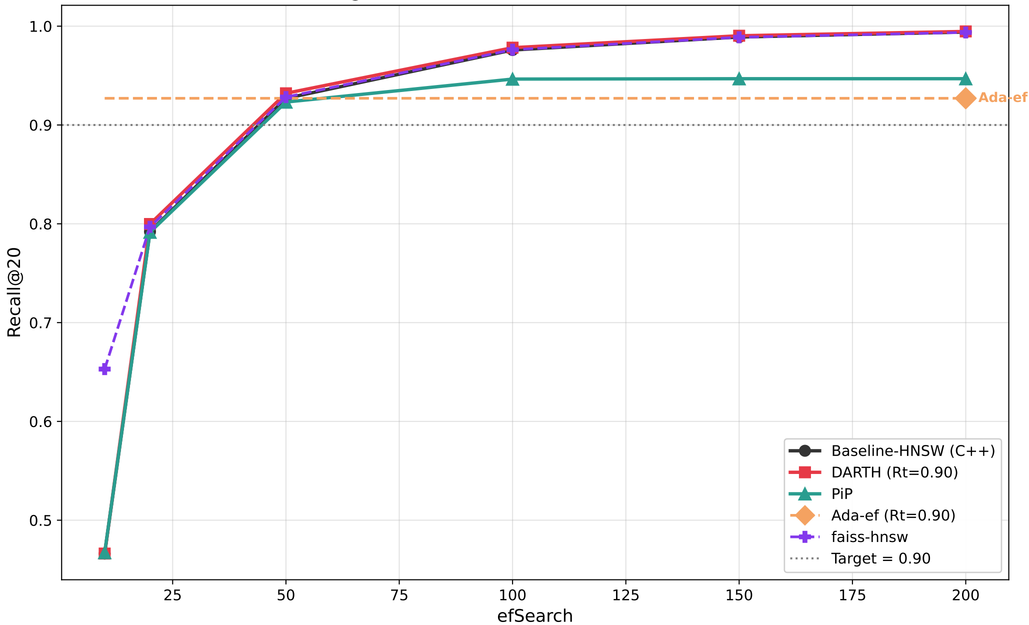
Recall@20 vs efSearch — sift1m (M=16, efC=128)
