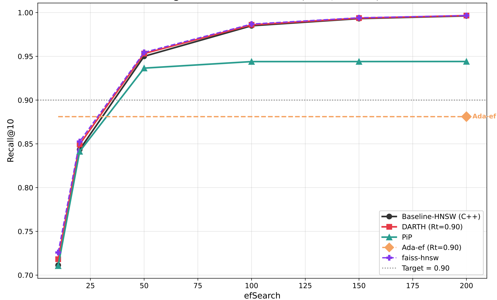
Recall@10 vs efSearch — sift1m (M=16, efC=200)
