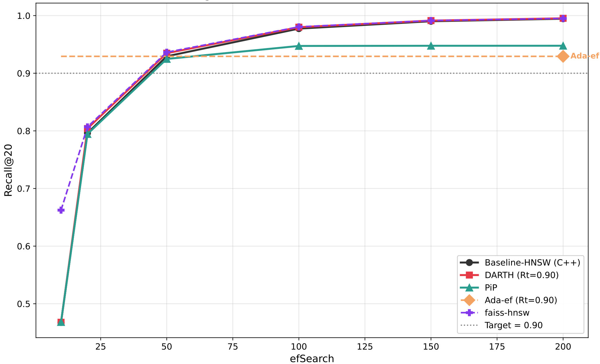
Recall@20 vs efSearch — sift1m (M=16, efC=200)
