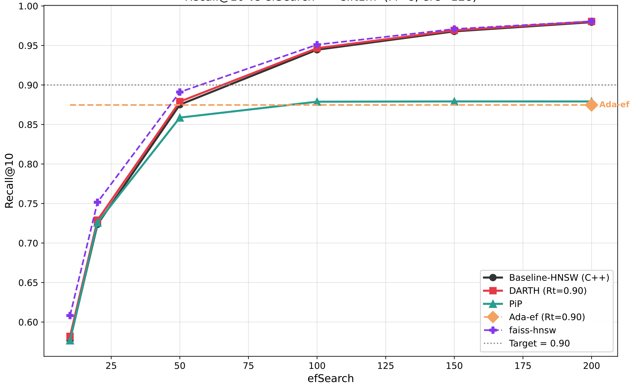
Recall@10 vs efSearch — sift1m (M=8, efC=128)
