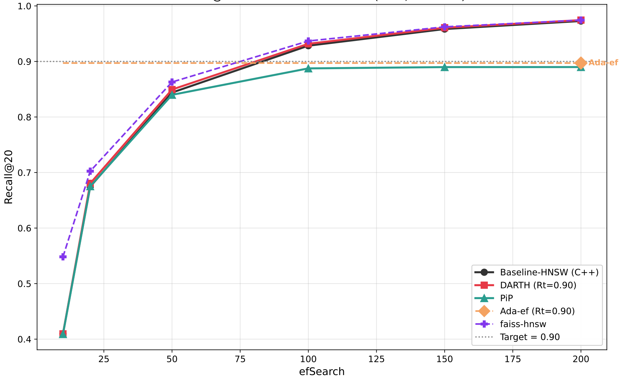
Recall@20 vs efSearch — sift1m (M=8, efC=128)
