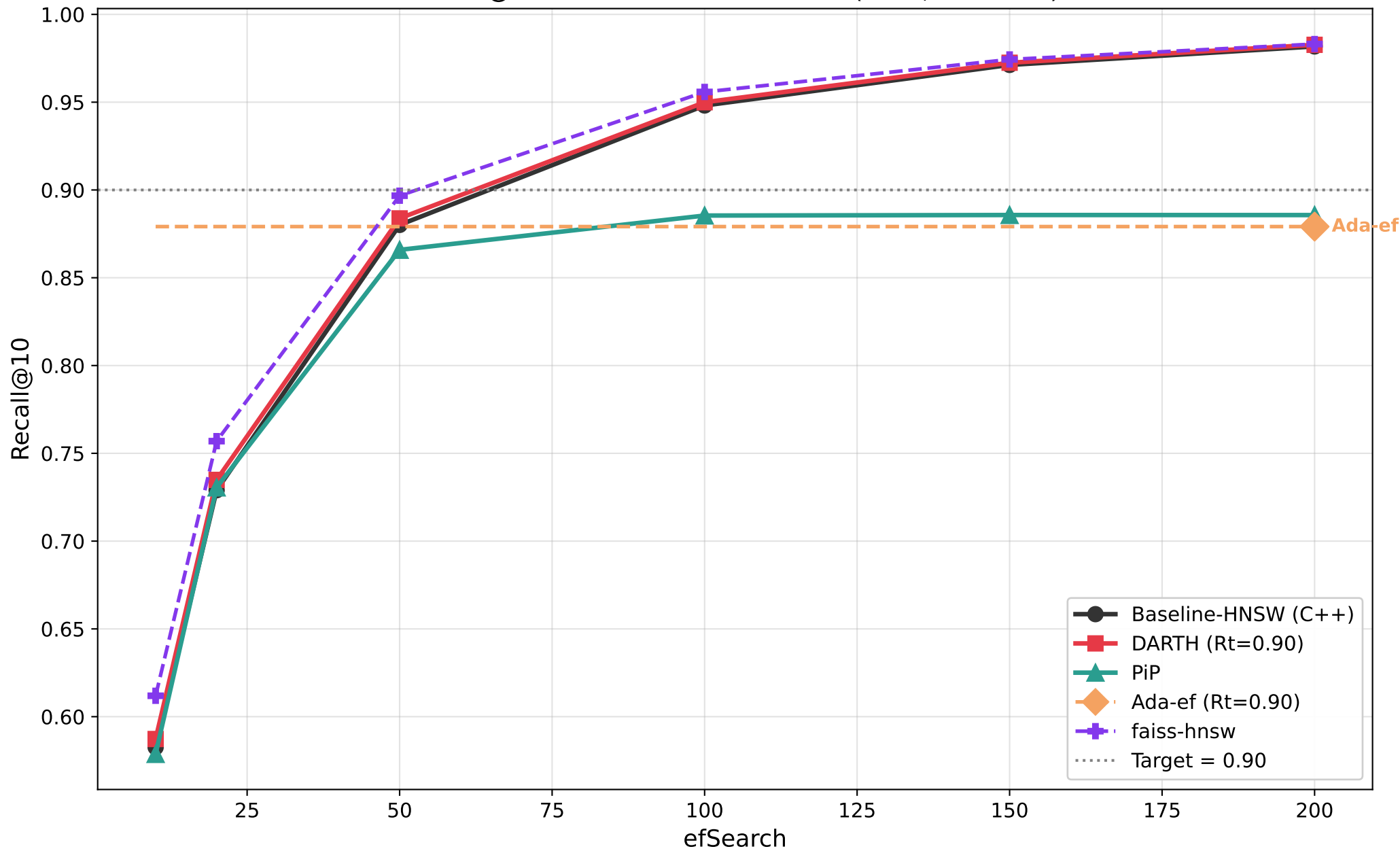
Recall@10 vs efSearch — sift1m (M=8, efC=200)
