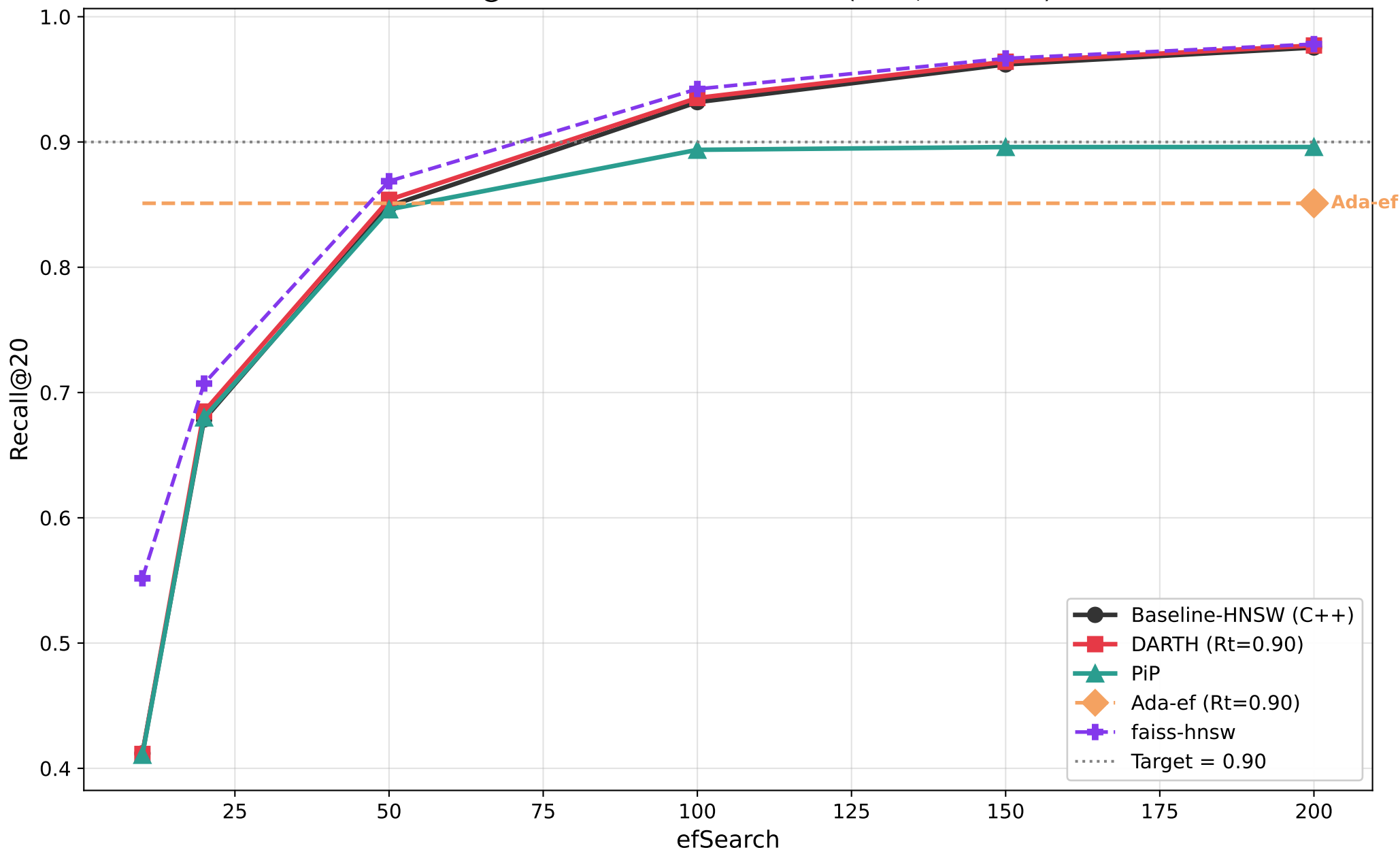
Recall@20 vs efSearch — sift1m (M=8, efC=200)
