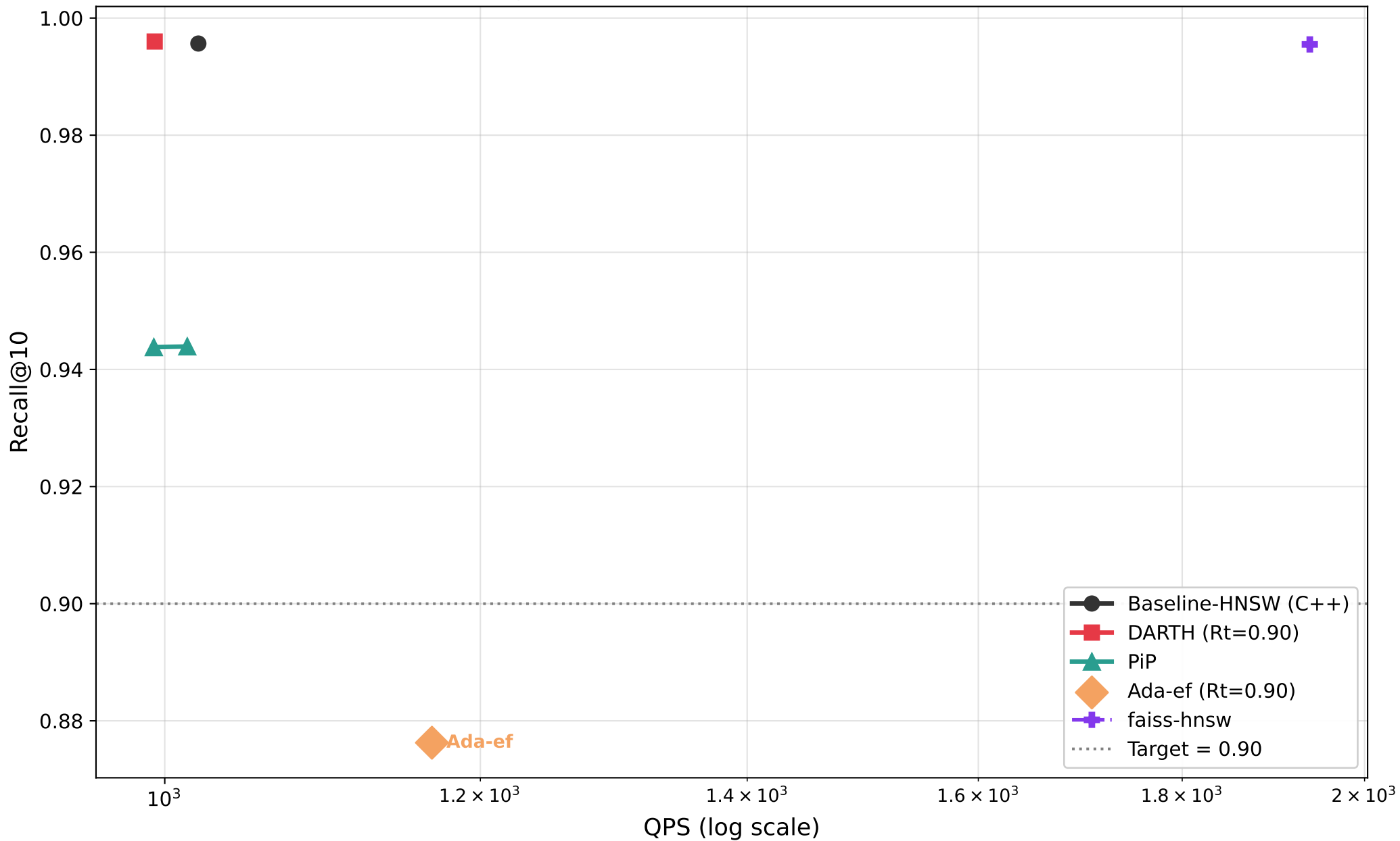
Recall@10 vs QPS — sift1m (M=16, efC=128)
