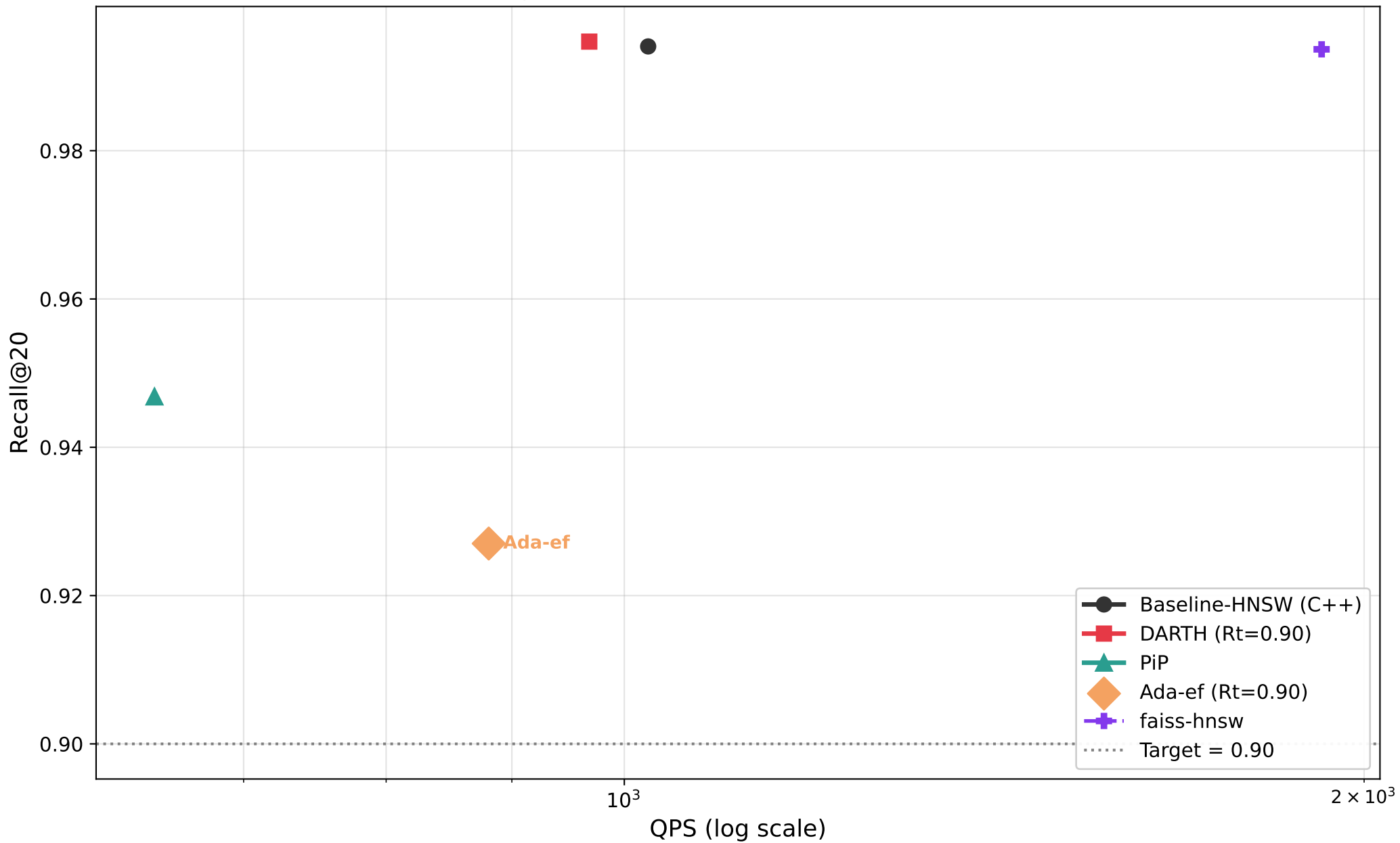
Recall@20 vs QPS — sift1m (M=16, efC=128)
