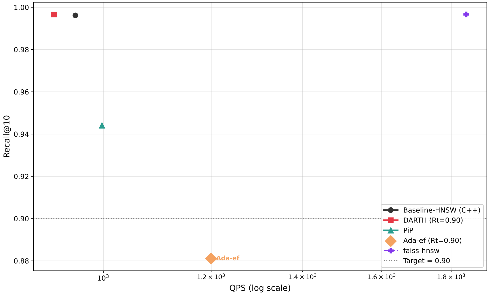
Recall@10 vs QPS — sift1m (M=16, efC=200)
