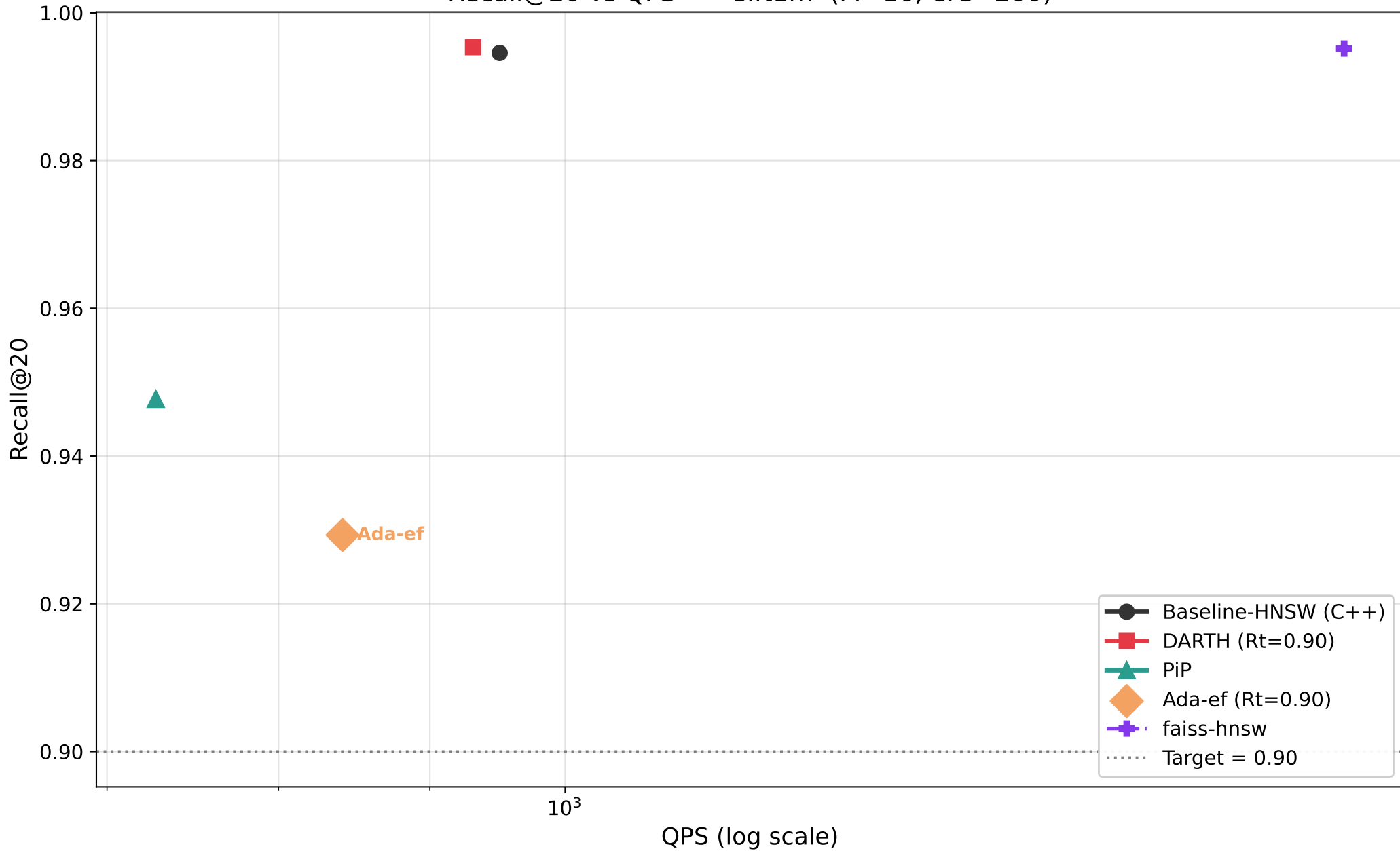
Recall@20 vs QPS — sift1m (M=16, efC=200)
