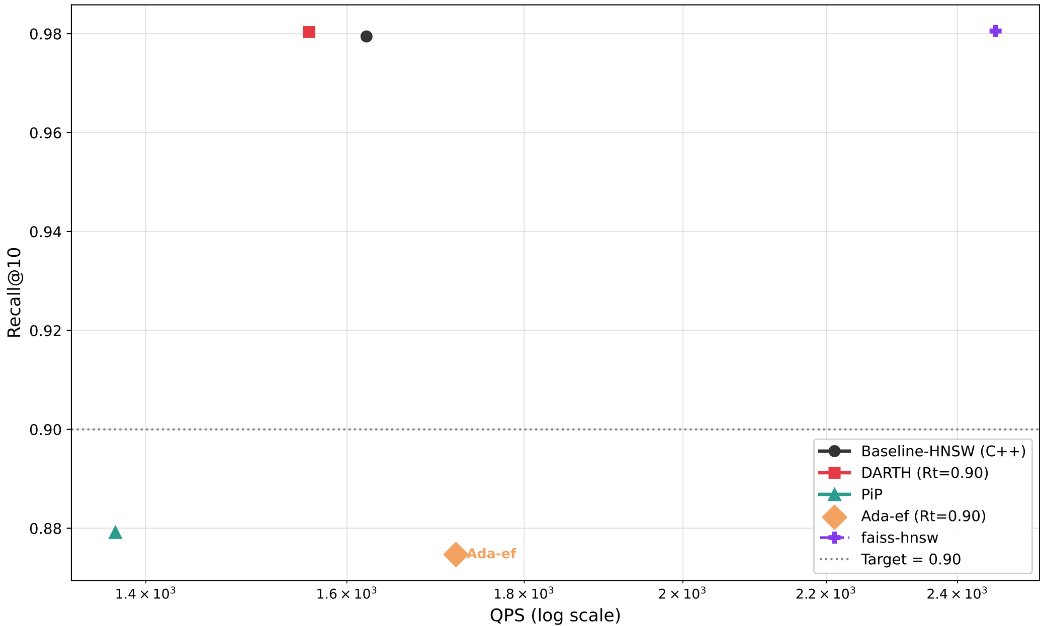
Recall@10 vs QPS — sift1m (M=8, efC=128)
