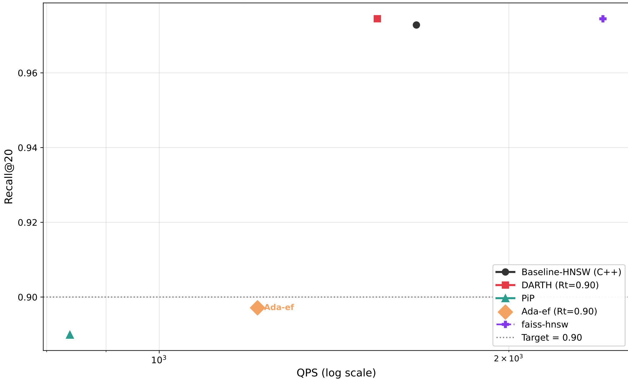
Recall@20 vs QPS — sift1m (M=8, efC=128)
