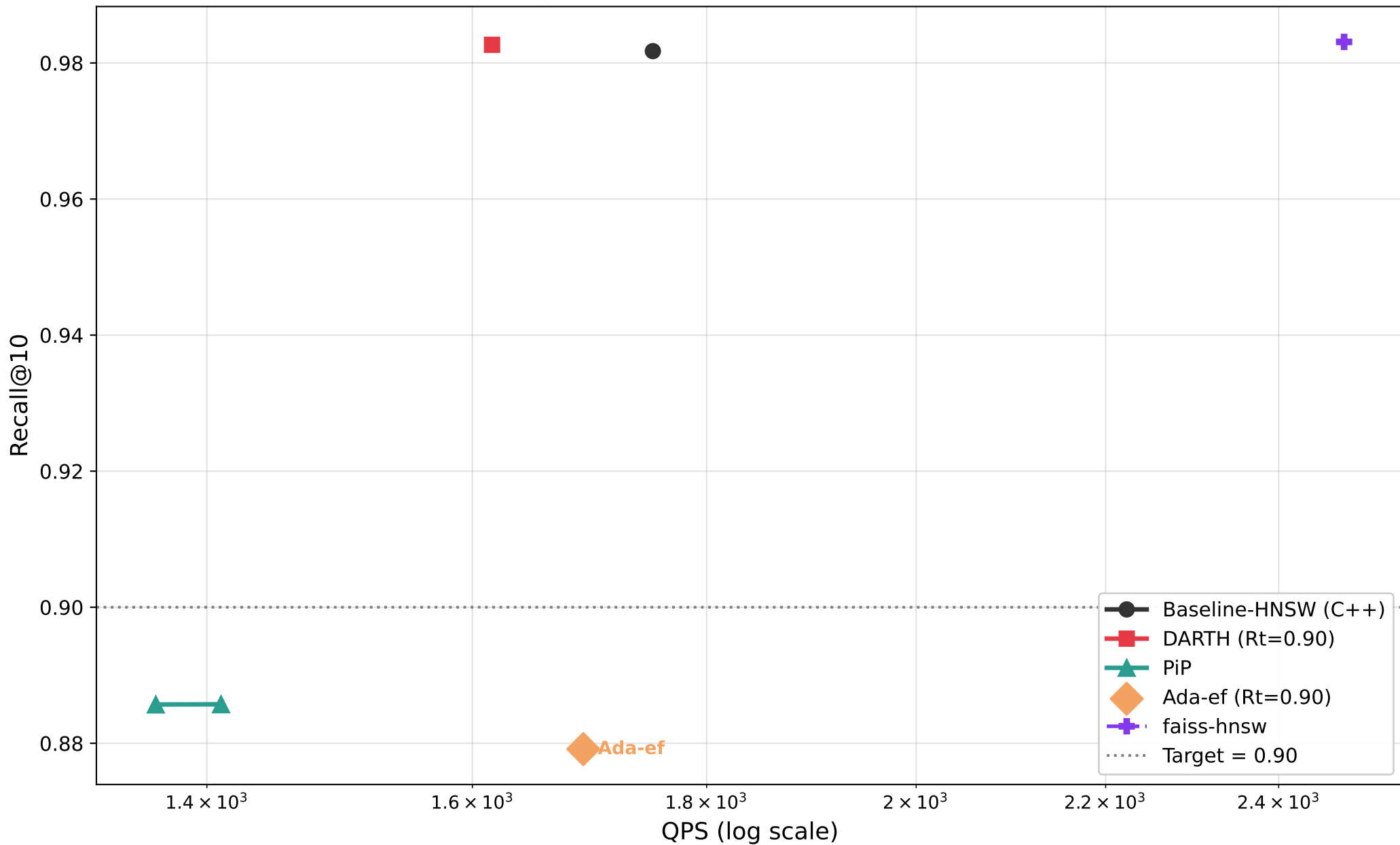
Recall@10 vs QPS — sift1m (M=8, efC=200)
