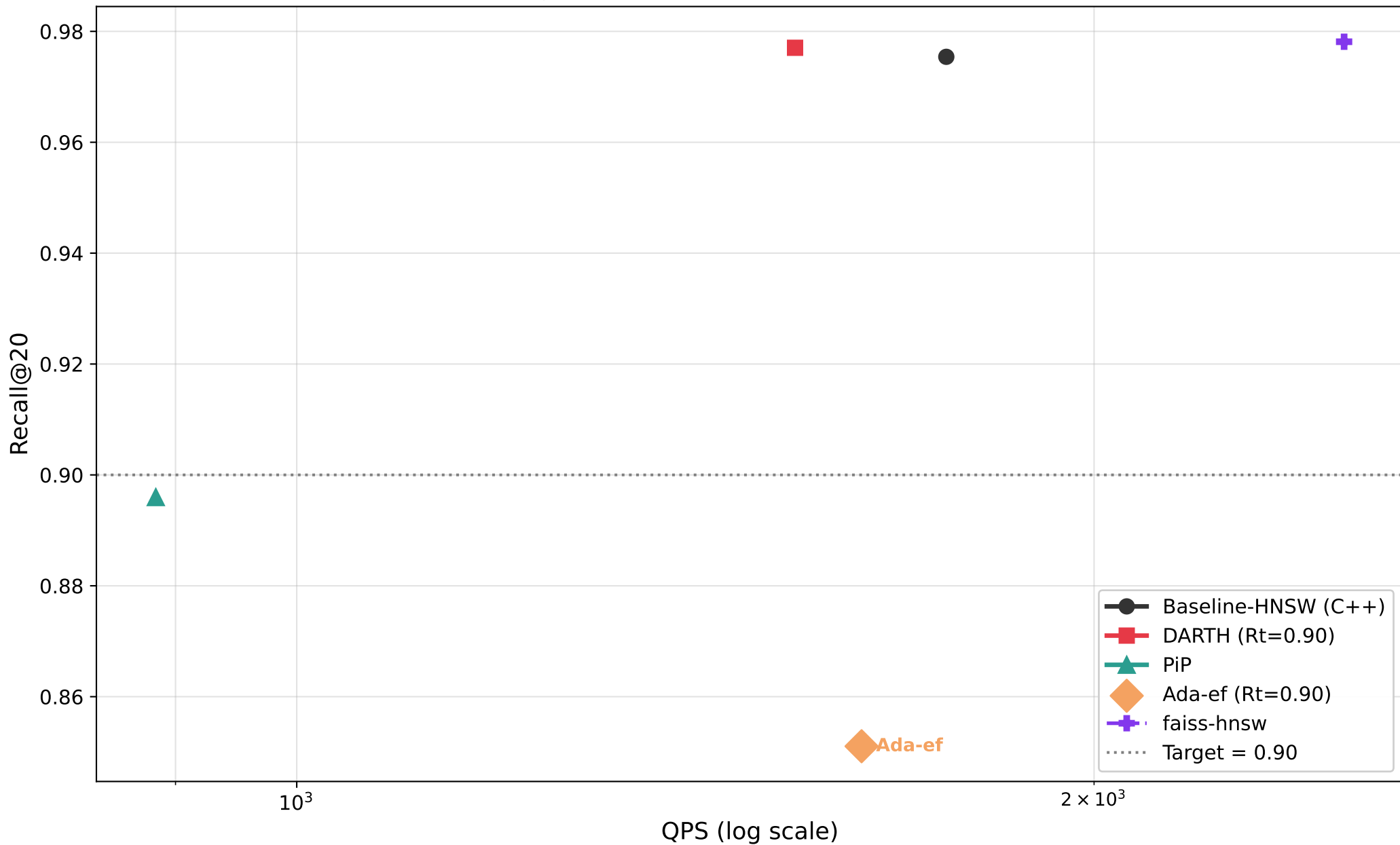
Recall@20 vs QPS — sift1m (M=8, efC=200)
