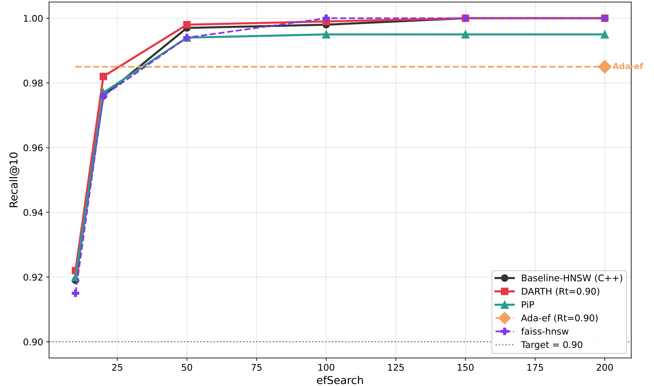
Recall@10 vs efSearch — siftsmall (M=16, efC=128)
