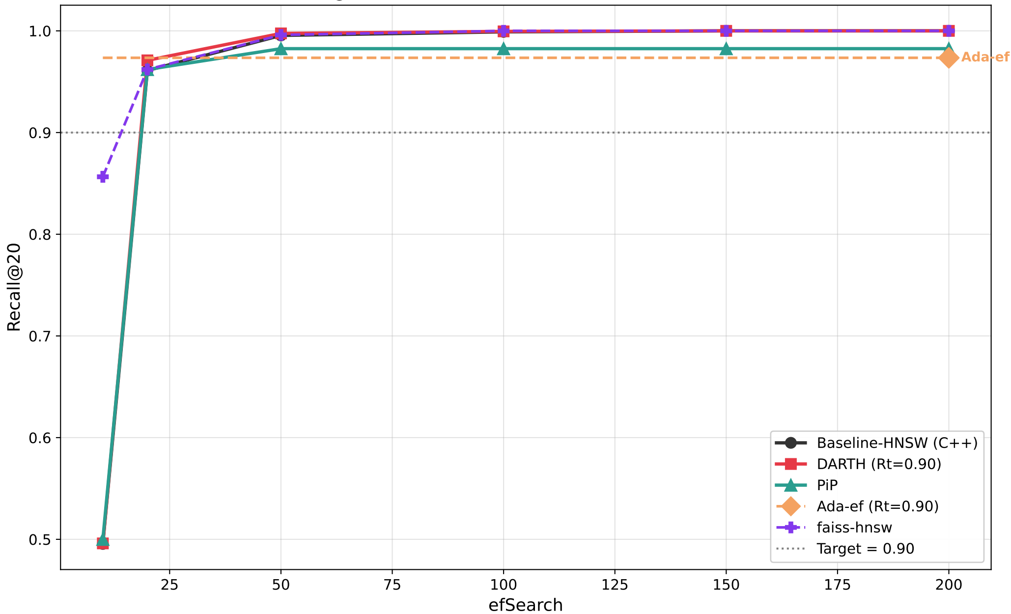
Recall@20 vs efSearch — siftsmall (M=16, efC=128)
