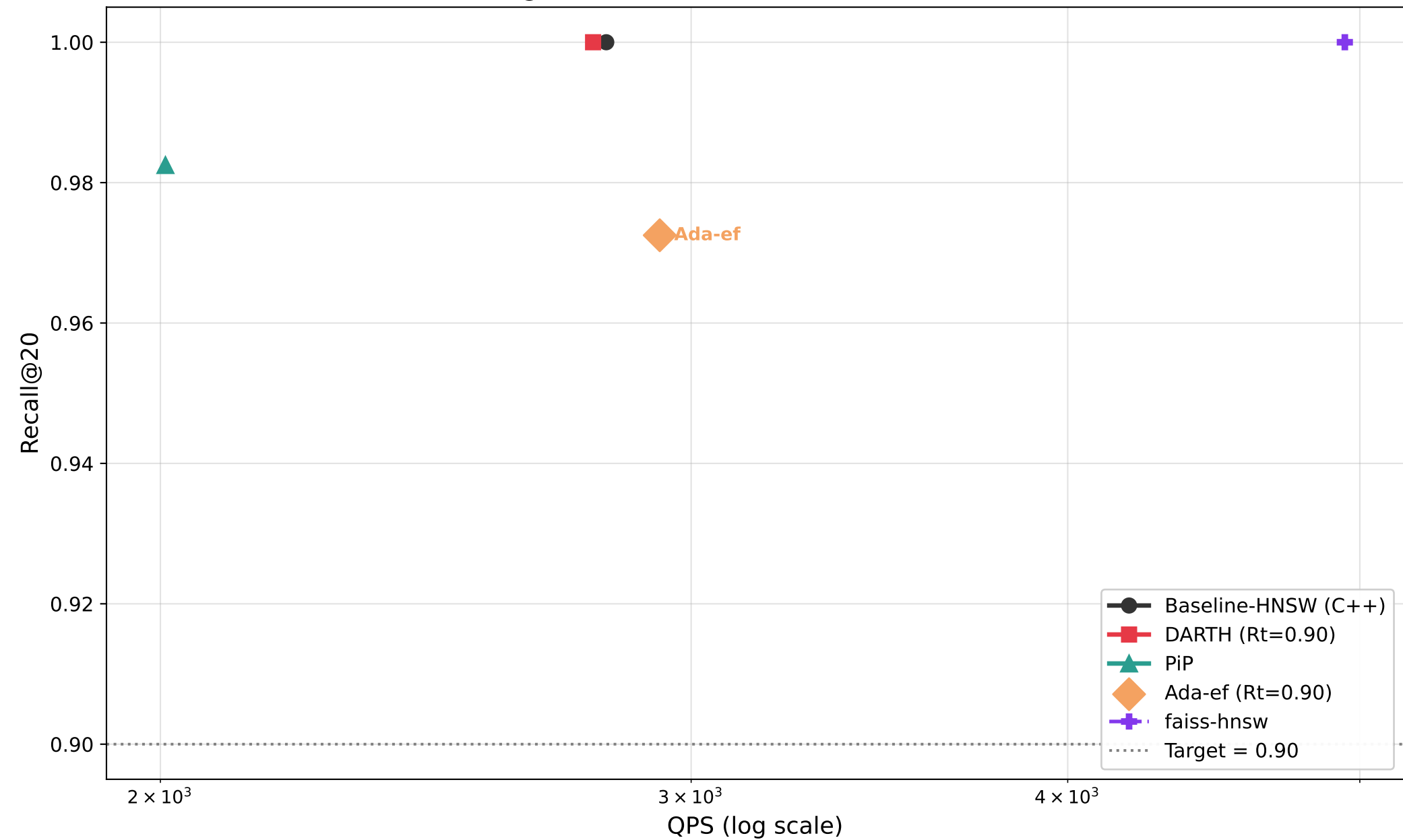
Recall@20 vs QPS — siftsmall (M=16, efC=200)
