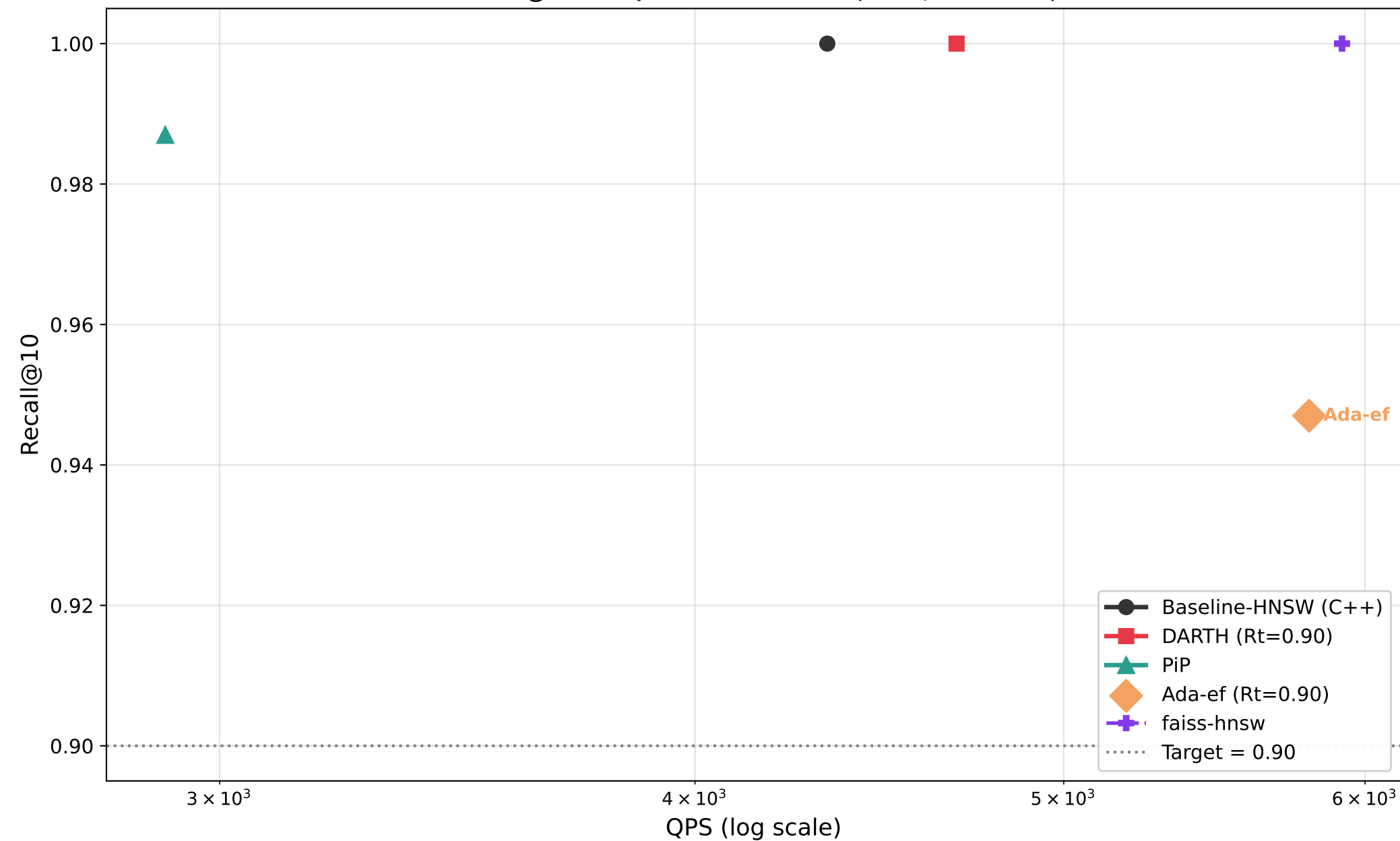
Recall@10 vs QPS — siftsmall (M=8, efC=200)
