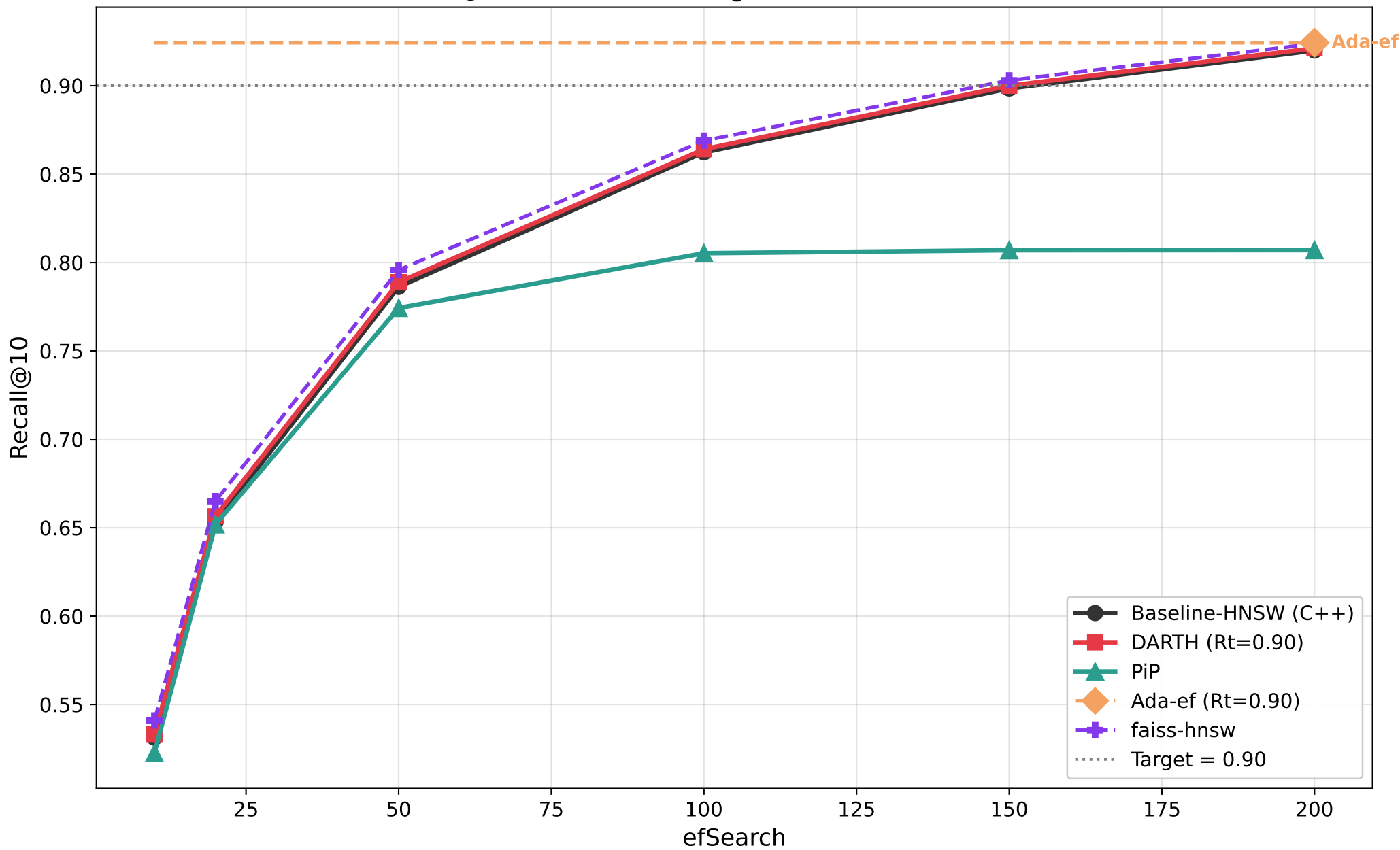
Recall@10 vs efSearch — glove100 (M=16, efC=200)
