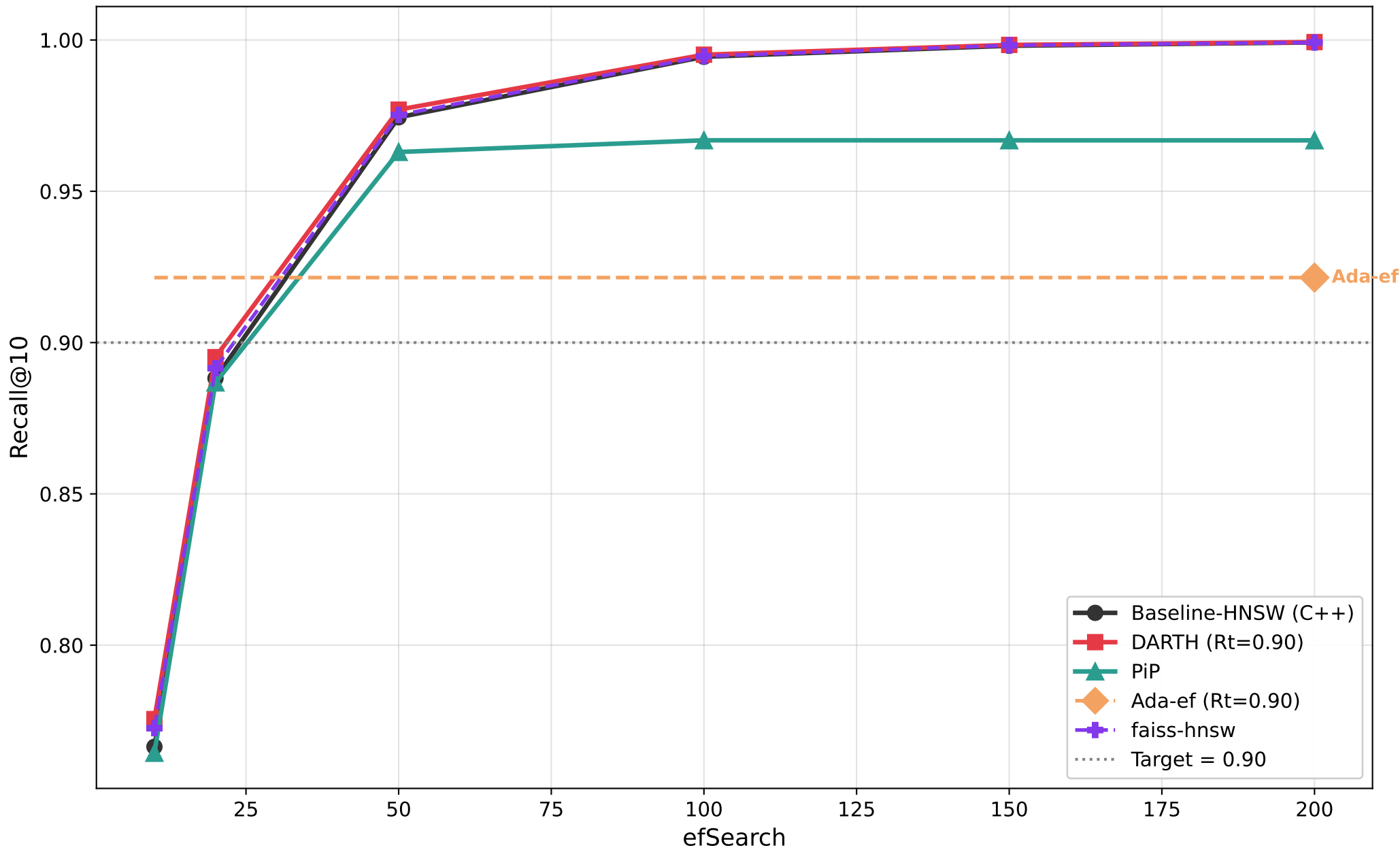
Recall@10 vs efSearch — sift128 (M=16, efC=200)
