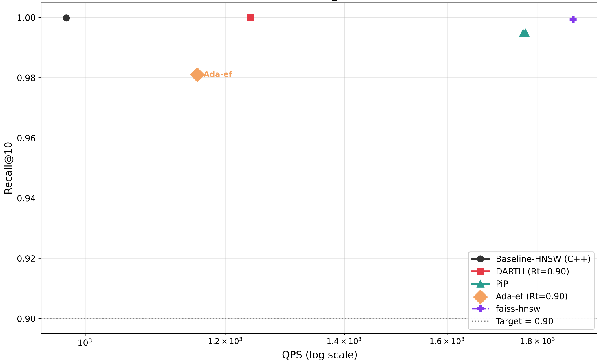
Recall@10 vs QPS — fashion_mnist (M=16, efC=200)
