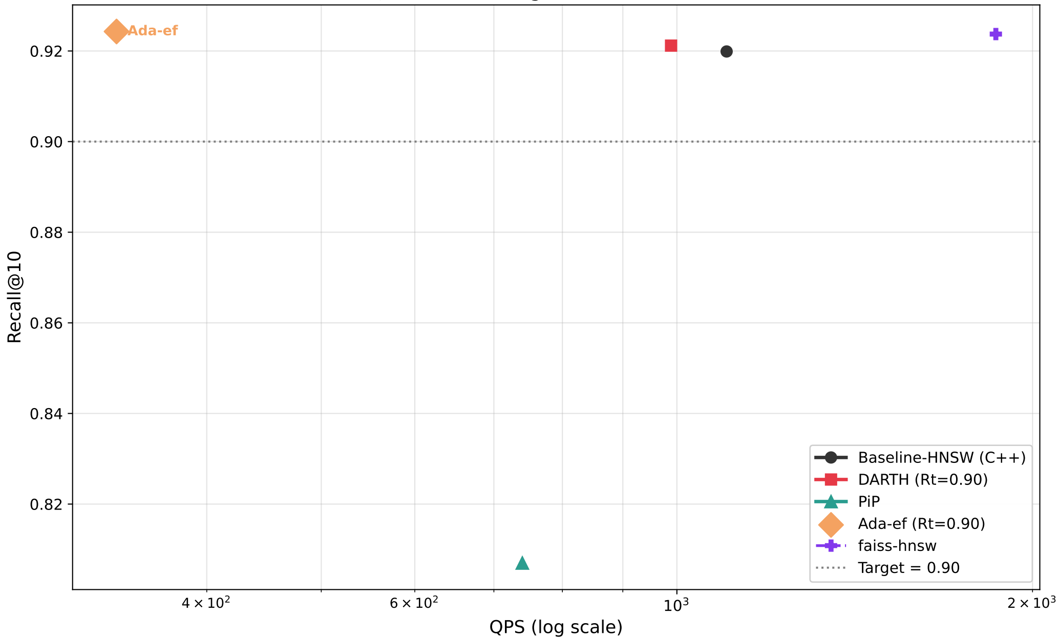
Recall@10 vs QPS — glove100 (M=16, efC=200)
