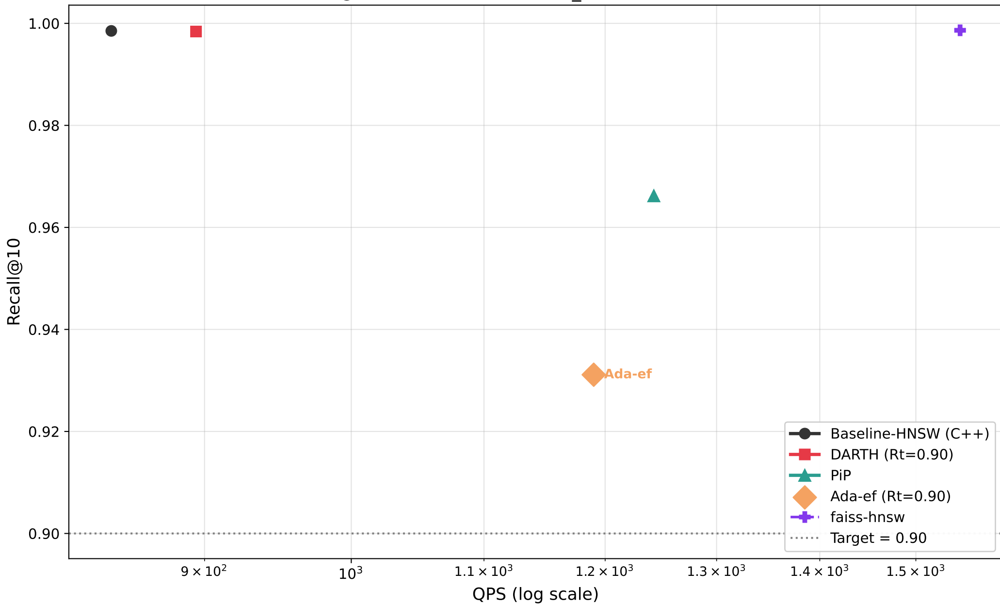
Recall@10 vs QPS — msmarco_text (M=16, efC=200)
