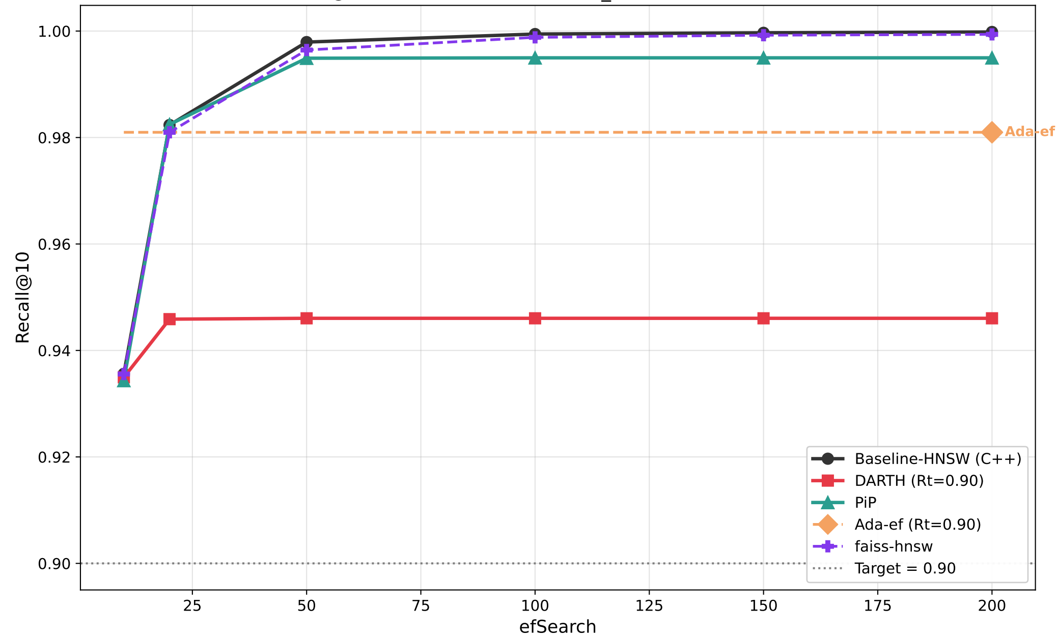
Recall@10 vs efSearch — fashion_mnist (M=16, efC=200)
