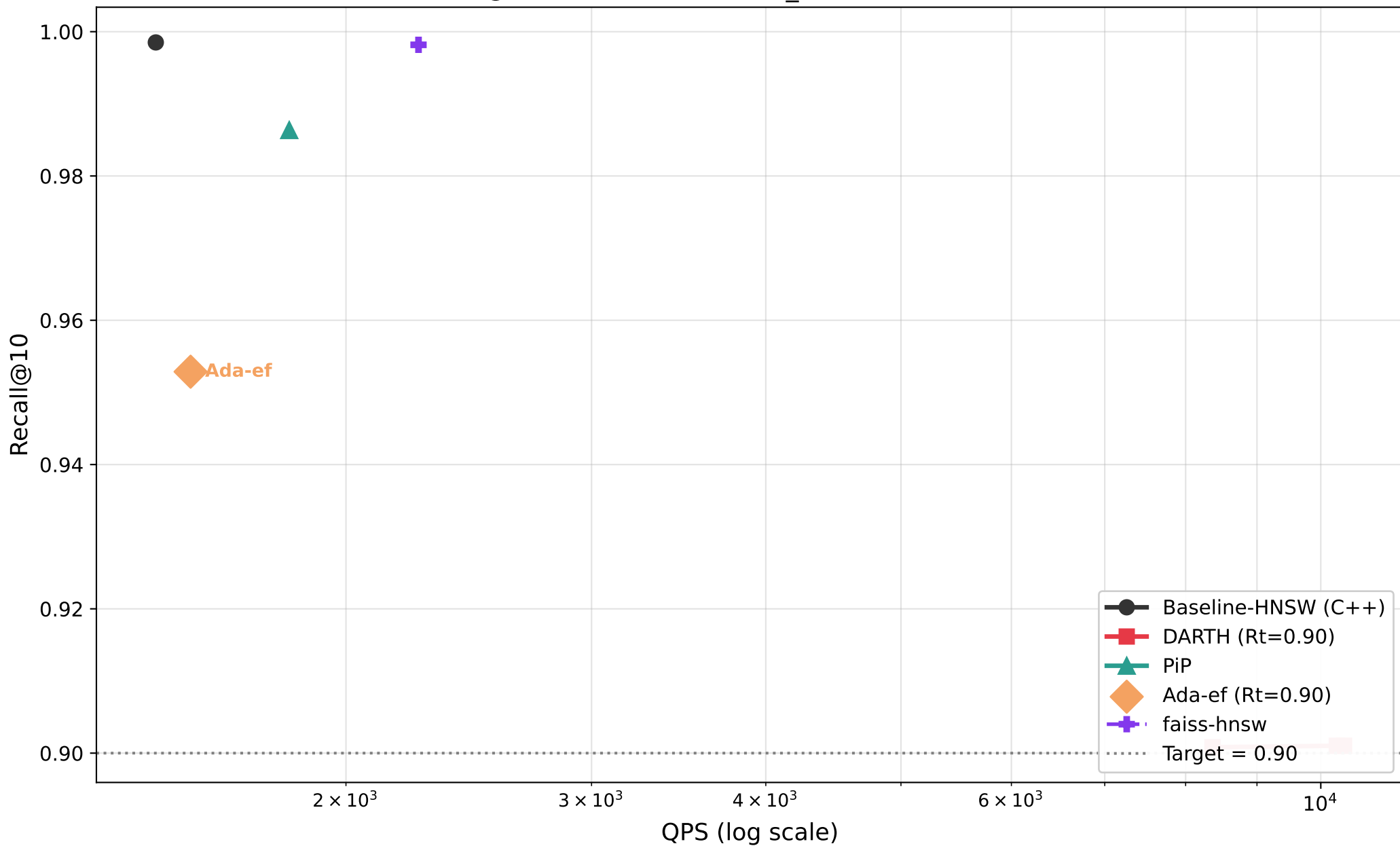
Recall@10 vs QPS — fashion_mnist (M=8, efC=128)
