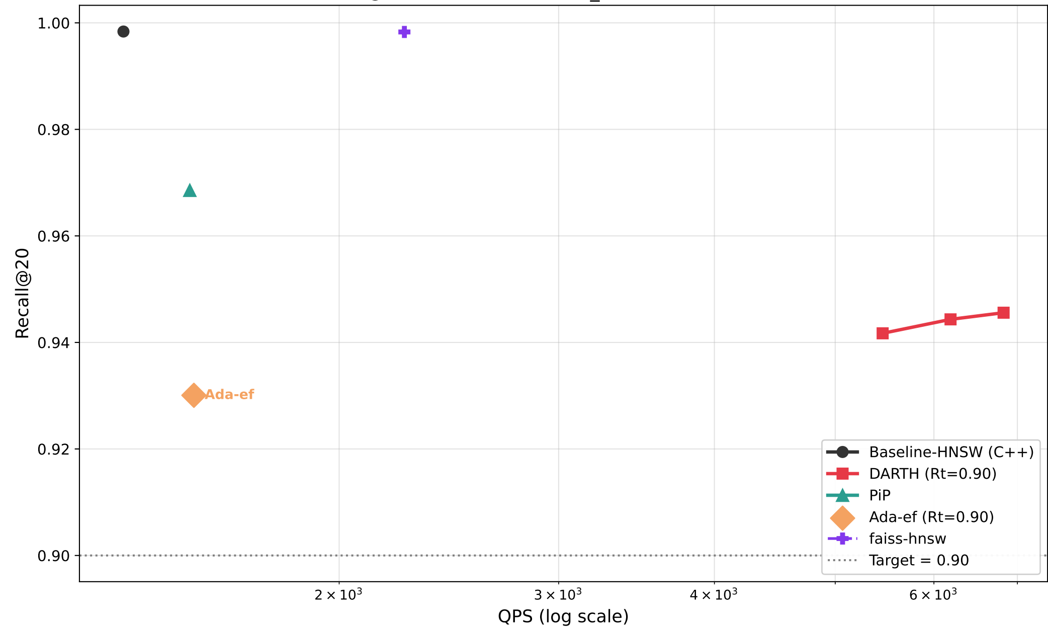
Recall@20 vs QPS — fashion_mnist (M=8, efC=128)
