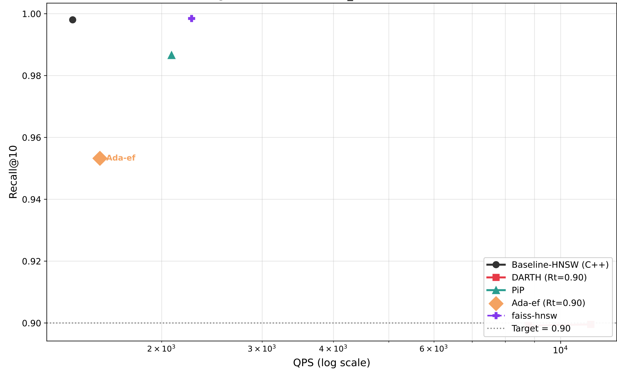
Recall@10 vs QPS — fashion_mnist (M=8, efC=200)
